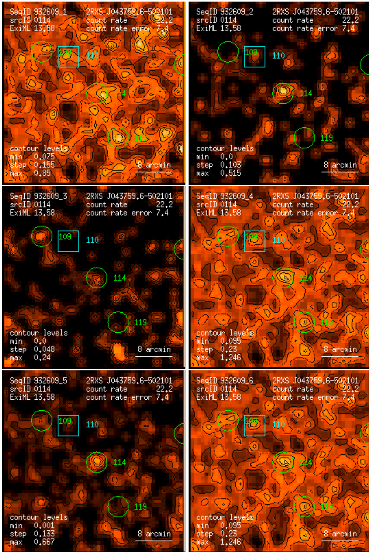
Figure 114: RASS 932609: detection 0114: band rate images, Gaussian filter: (1) PSPC channels 11 – 41, (2) 52 – 90, (3) 91 – 201, (4) 11 – 235, (5) 52 – 201, (6) 11 – 201. Broad band rates in counts/ks. Band rate contour levels in counts/ks/arcmin 2 .
