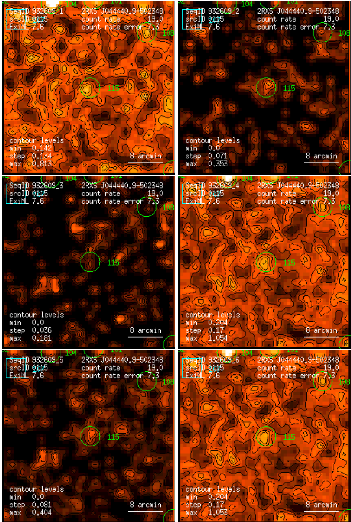
Figure 115: RASS 932609: detection 0115: band rate images, Gaussian filter: (1) PSPC channels 11 – 41, (2) 52 – 90, (3) 91 – 201, (4) 11 – 235, (5) 52 – 201, (6) 11 – 201. Broad band rates in counts/ks. Band rate contour levels in counts/ks/arcmin 2 .
