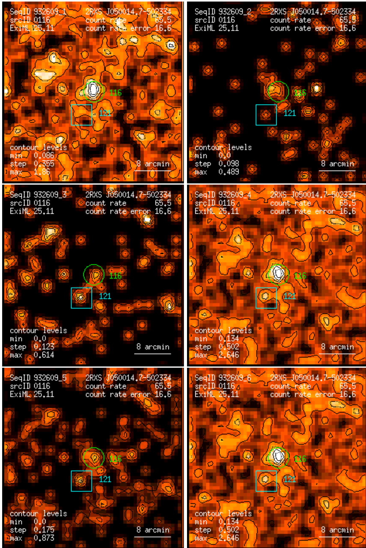
Figure 116: RASS 932609: detection 0116: band rate images, Gaussian filter: (1) PSPC channels 11 – 41, (2) 52 – 90, (3) 91 – 201, (4) 11 – 235, (5) 52 – 201, (6) 11 – 201. Broad band rates in counts/ks. Band rate contour levels in counts/ks/arcmin 2 .
