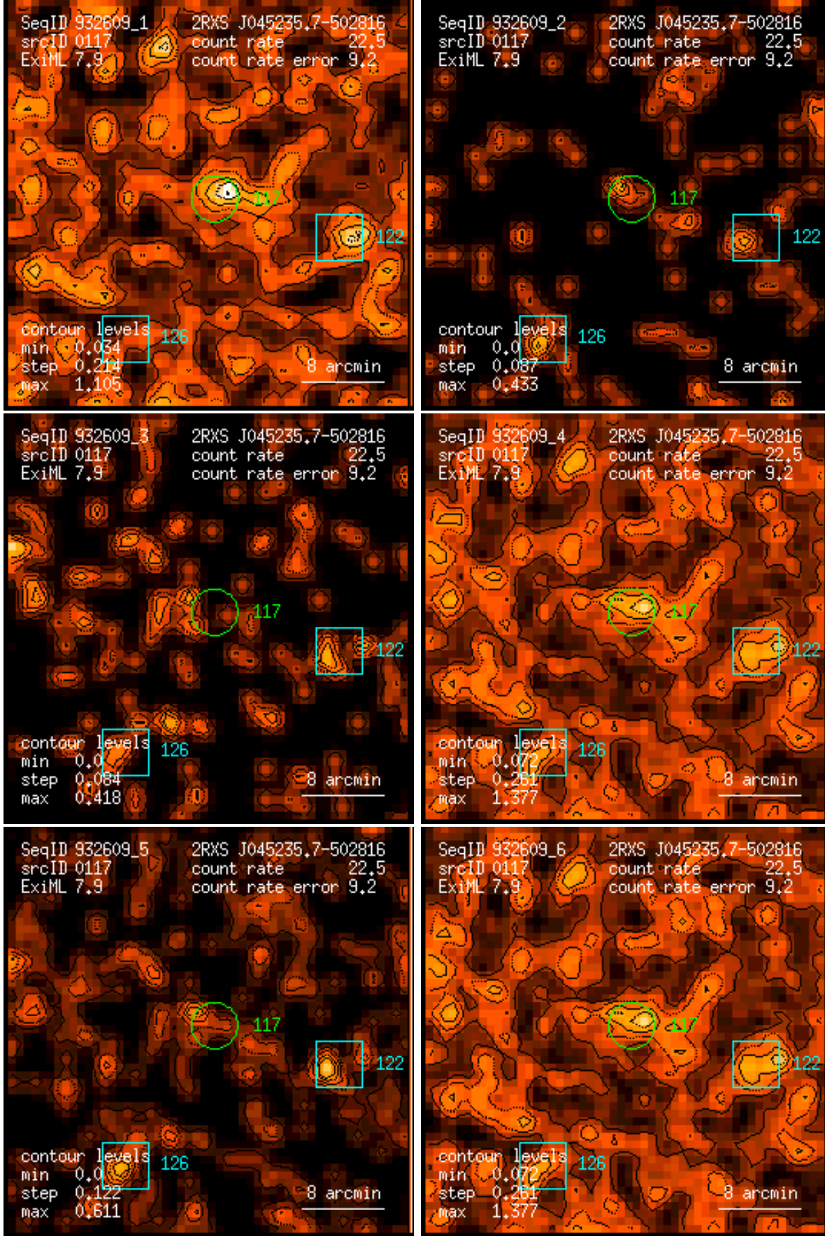
Figure 117: RASS 932609: detection 0117: band rate images, Gaussian filter: (1) PSPC channels 11 – 41, (2) 52 – 90, (3) 91 – 201, (4) 11 – 235, (5) 52 – 201, (6) 11 – 201. Broad band rates in counts/ks. Band rate contour levels in counts/ks/arcmin 2 .
