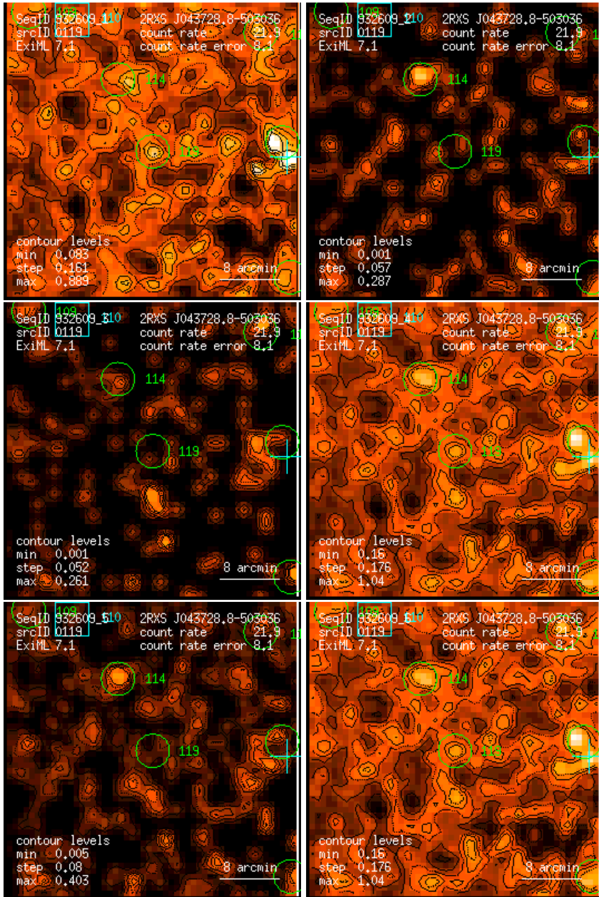
Figure 119: RASS 932609: detection 0119: band rate images, Gaussian filter: (1) PSPC channels 11 – 41, (2) 52 – 90, (3) 91 – 201, (4) 11 – 235, (5) 52 – 201, (6) 11 – 201. Broad band rates in counts/ks. Band rate contour levels in counts/ks/arcmin 2 .
