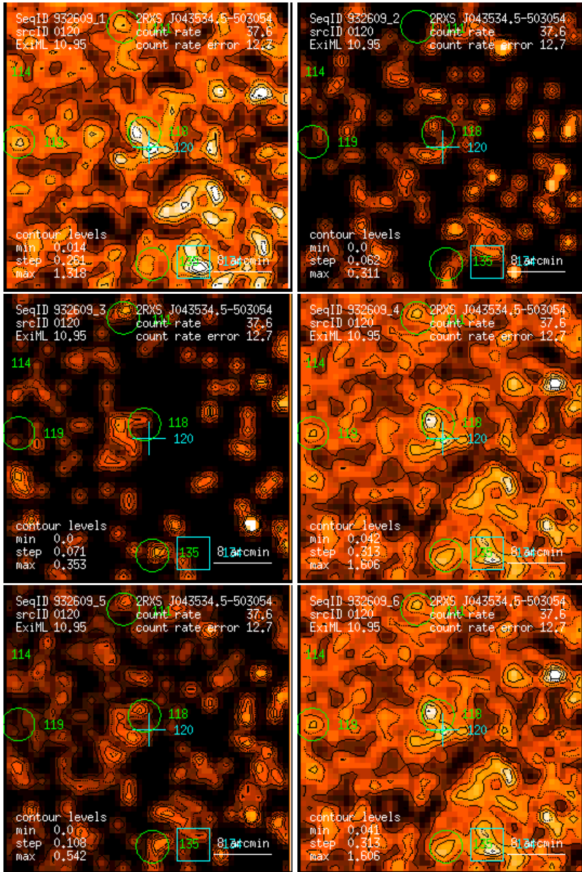
Figure 120: RASS 932609: detection 0120: band rate images, Gaussian filter: (1) PSPC channels 11 – 41, (2) 52 – 90, (3) 91 – 201, (4) 11 – 235, (5) 52 – 201, (6) 11 – 201. Broad band rates in counts/ks. Band rate contour levels in counts/ks/arcmin 2 .
