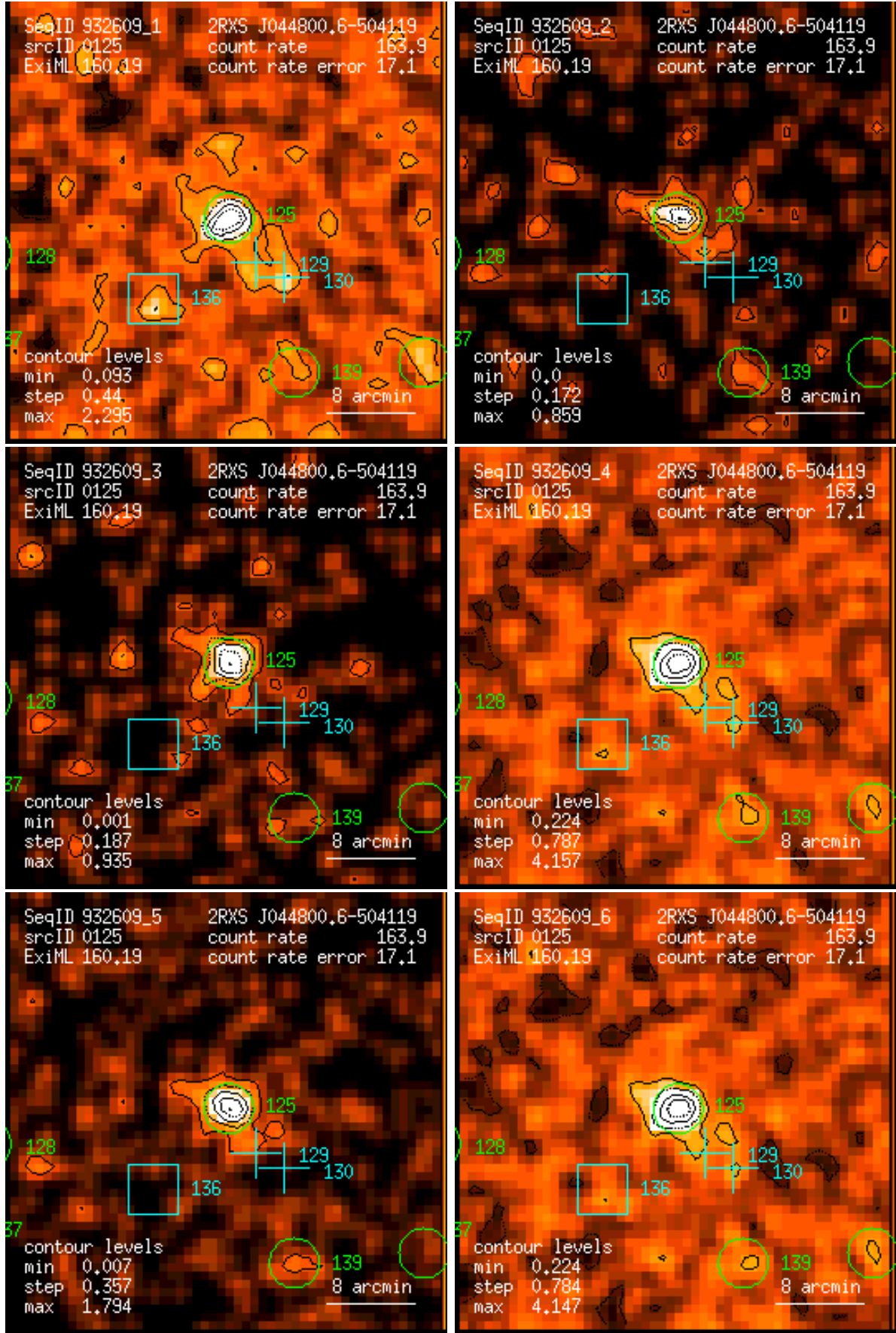
Figure 125: RASS 932609: detection 0125: band rate images, Gaussian filter: (1) PSPC channels 11 – 41, (2) 52 – 90, (3) 91 – 201, (4) 11 – 235, (5) 52 – 201, (6) 11 – 201. Broad band rates in counts/ks. Band rate contour levels in counts/ks/arcmin 2 .
