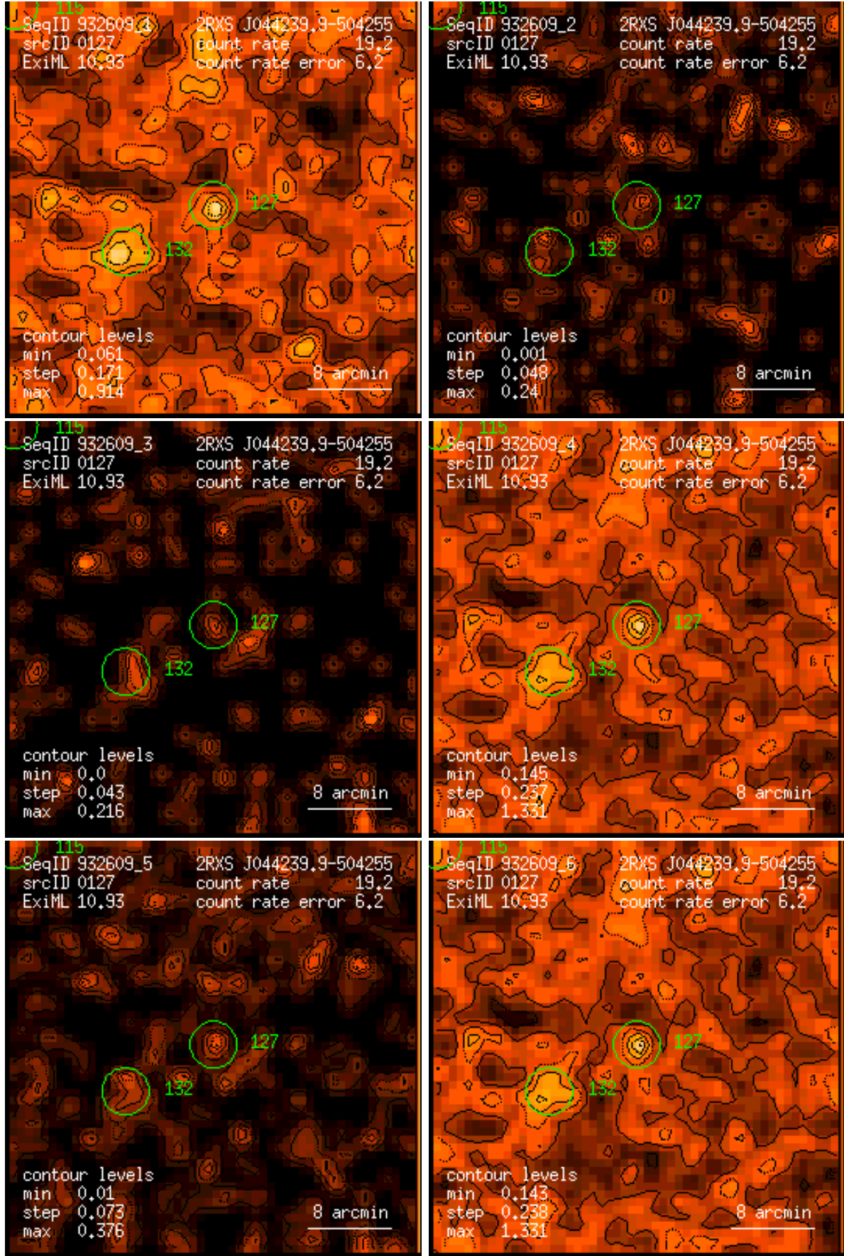
Figure 127: RASS 932609: detection 0127: band rate images, Gaussian filter: (1) PSPC channels 11 – 41, (2) 52 – 90, (3) 91 – 201, (4) 11 – 235, (5) 52 – 201, (6) 11 – 201. Broad band rates in counts/ks. Band rate contour levels in counts/ks/arcmin 2 .
