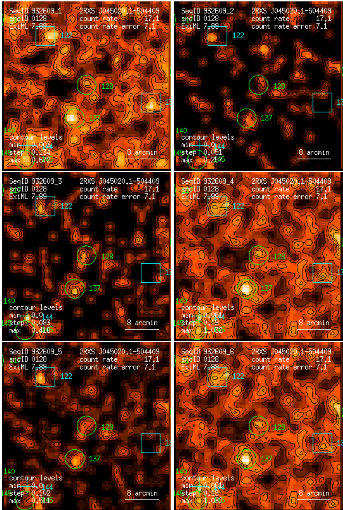
Figure 128: RASS 932609: detection 0128: band rate images, Gaussian filter: (1) PSPC channels 11 – 41, (2) 52 – 90, (3) 91 – 201, (4) 11 – 235, (5) 52 – 201, (6) 11 – 201. Broad band rates in counts/ks. Band rate contour levels in counts/ks/arcmin 2 .
