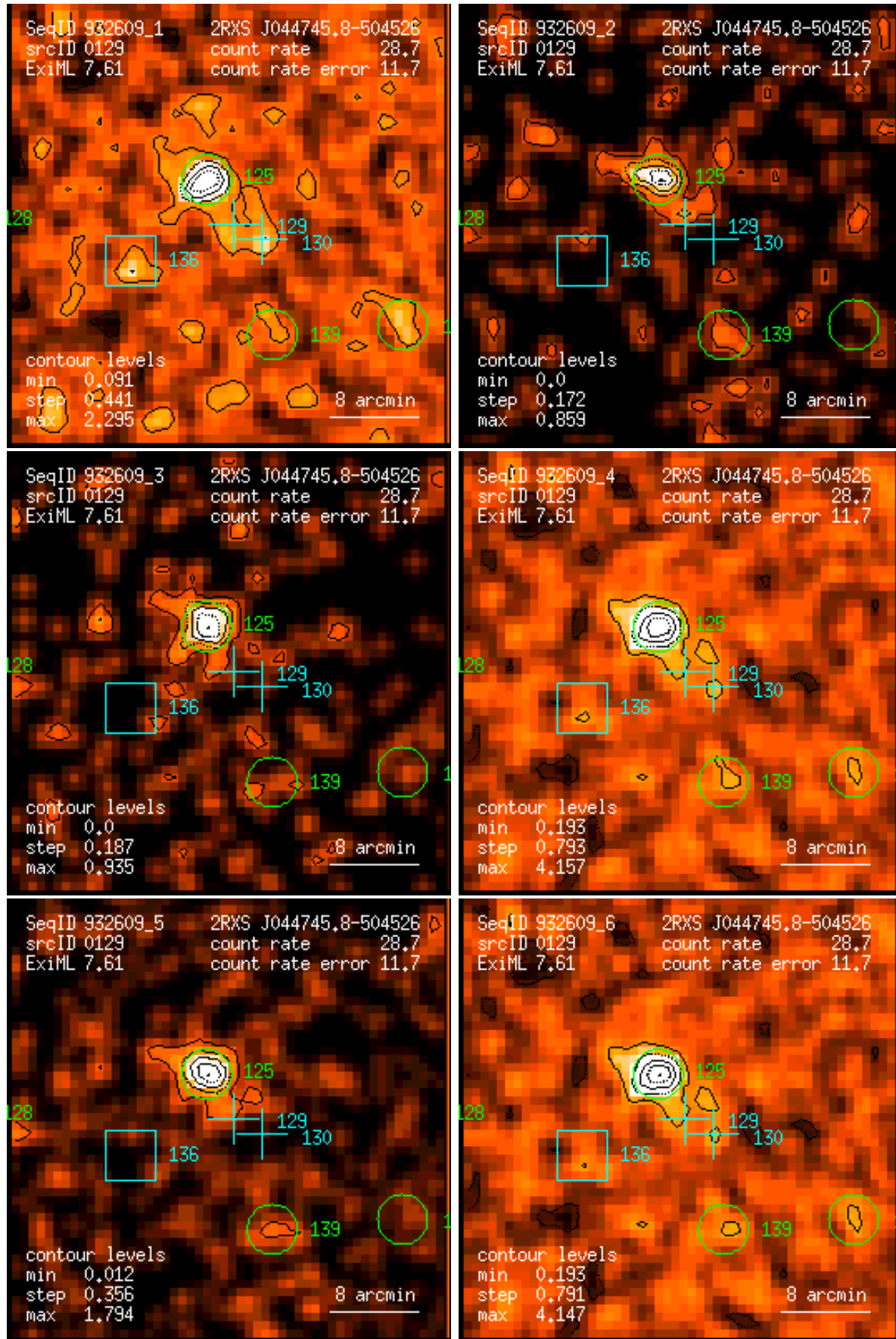
Figure 129: RASS 932609: detection 0129: band rate images, Gaussian filter: (1) PSPC channels 11 – 41, (2) 52 – 90, (3) 91 – 201, (4) 11 – 235, (5) 52 – 201, (6) 11 – 201. Broad band rates in counts/ks. Band rate contour levels in counts/ks/arcmin 2 .
