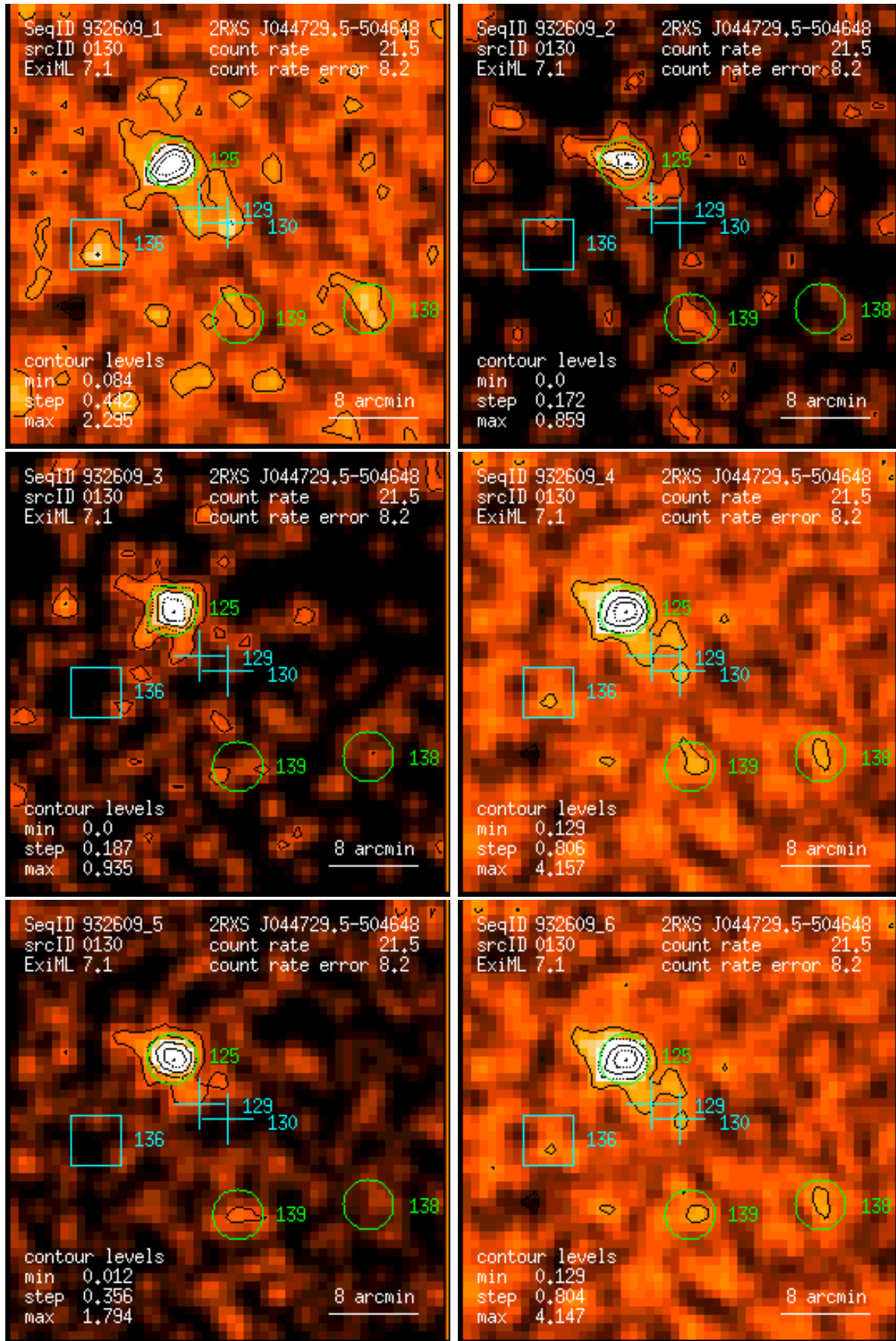
Figure 130: RASS 932609: detection 0130: band rate images, Gaussian filter: (1) PSPC channels 11 – 41, (2) 52 – 90, (3) 91 – 201, (4) 11 – 235, (5) 52 – 201, (6) 11 – 201. Broad band rates in counts/ks. Band rate contour levels in counts/ks/arcmin 2 .
