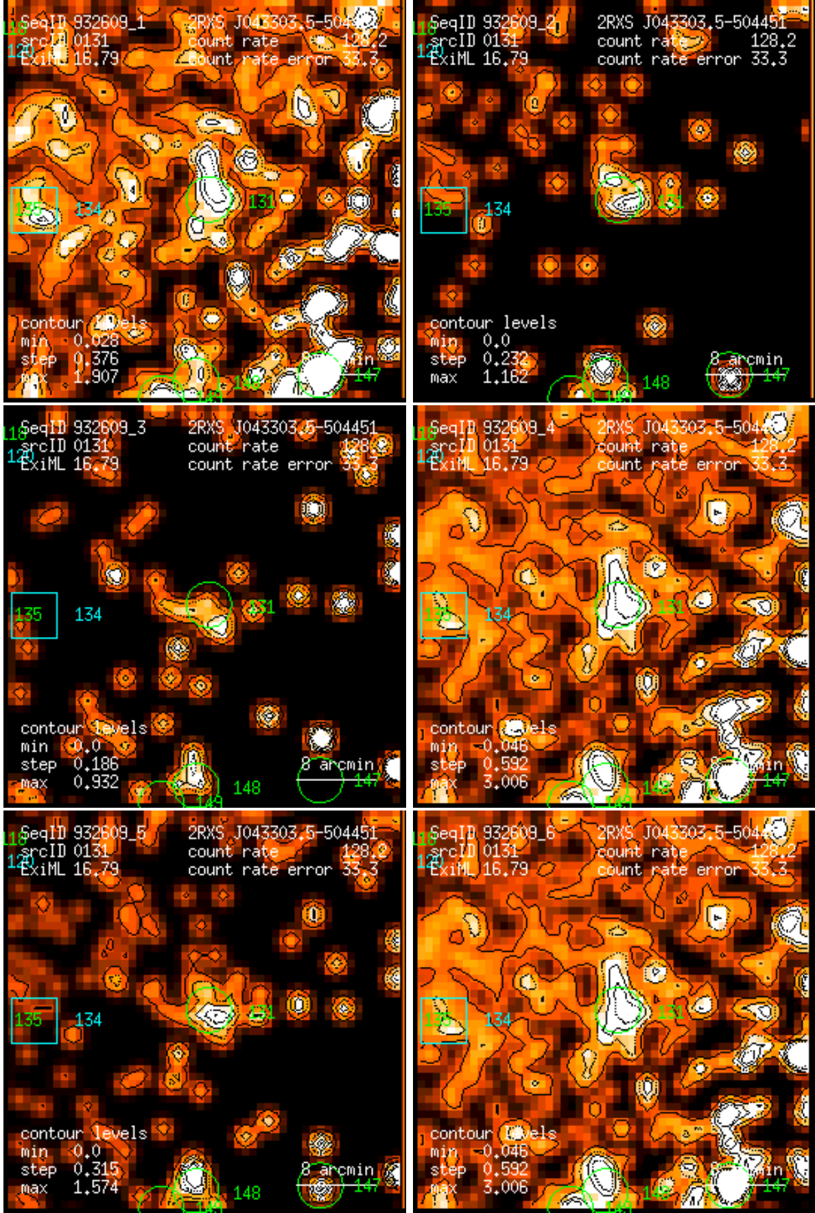
Figure 131: RASS 932609: detection 0131: band rate images, Gaussian filter: (1) PSPC channels 11 – 41, (2) 52 – 90, (3) 91 – 201, (4) 11 – 235, (5) 52 – 201, (6) 11 – 201. Broad band rates in counts/ks. Band rate contour levels in counts/ks/arcmin 2 .
