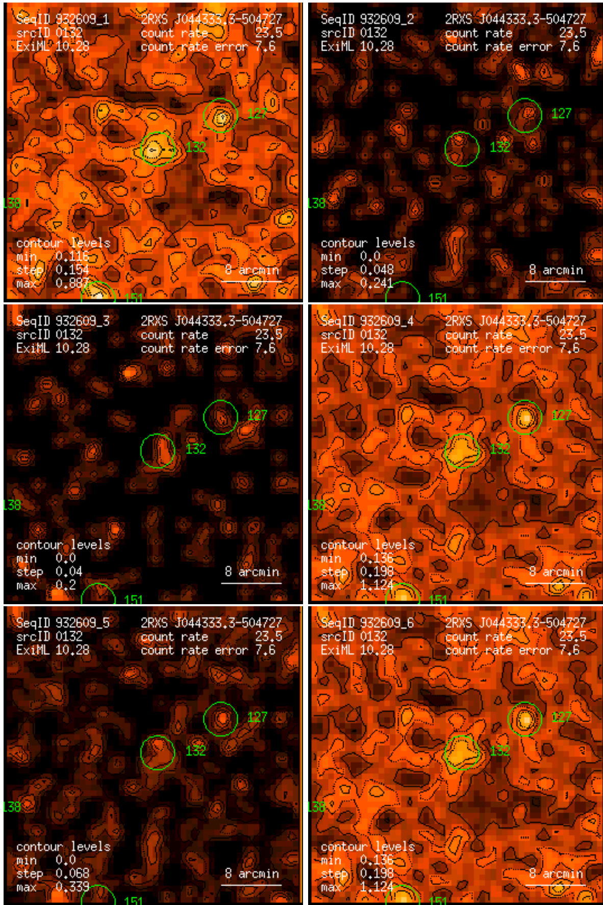
Figure 132: RASS 932609: detection 0132: band rate images, Gaussian filter: (1) PSPC channels 11 – 41, (2) 52 – 90, (3) 91 – 201, (4) 11 – 235, (5) 52 – 201, (6) 11 – 201. Broad band rates in counts/ks. Band rate contour levels in counts/ks/arcmin 2 .
