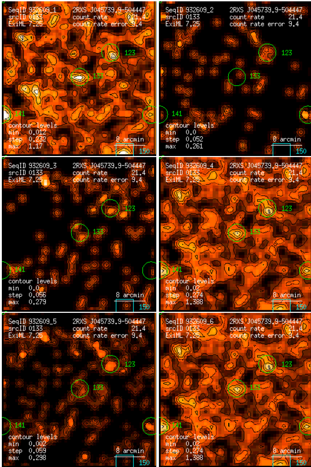
Figure 133: RASS 932609: detection 0133: band rate images, Gaussian filter: (1) PSPC channels 11 – 41, (2) 52 – 90, (3) 91 – 201, (4) 11 – 235, (5) 52 – 201, (6) 11 – 201. Broad band rates in counts/ks. Band rate contour levels in counts/ks/arcmin 2 .
