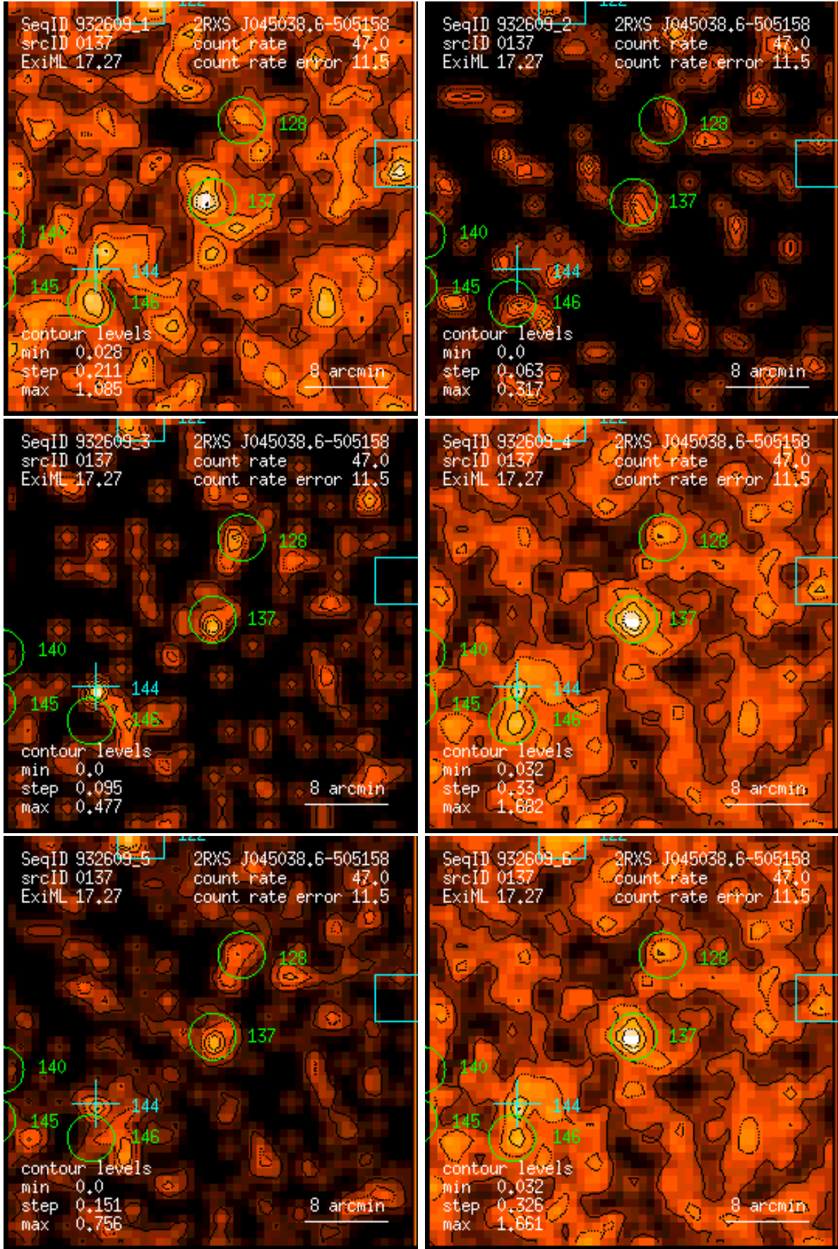
Figure 137: RASS 932609: detection 0137: band rate images, Gaussian filter: (1) PSPC channels 11 – 41, (2) 52 – 90, (3) 91 – 201, (4) 11 – 235, (5) 52 – 201, (6) 11 – 201. Broad band rates in counts/ks. Band rate contour levels in counts/ks/arcmin 2 .
