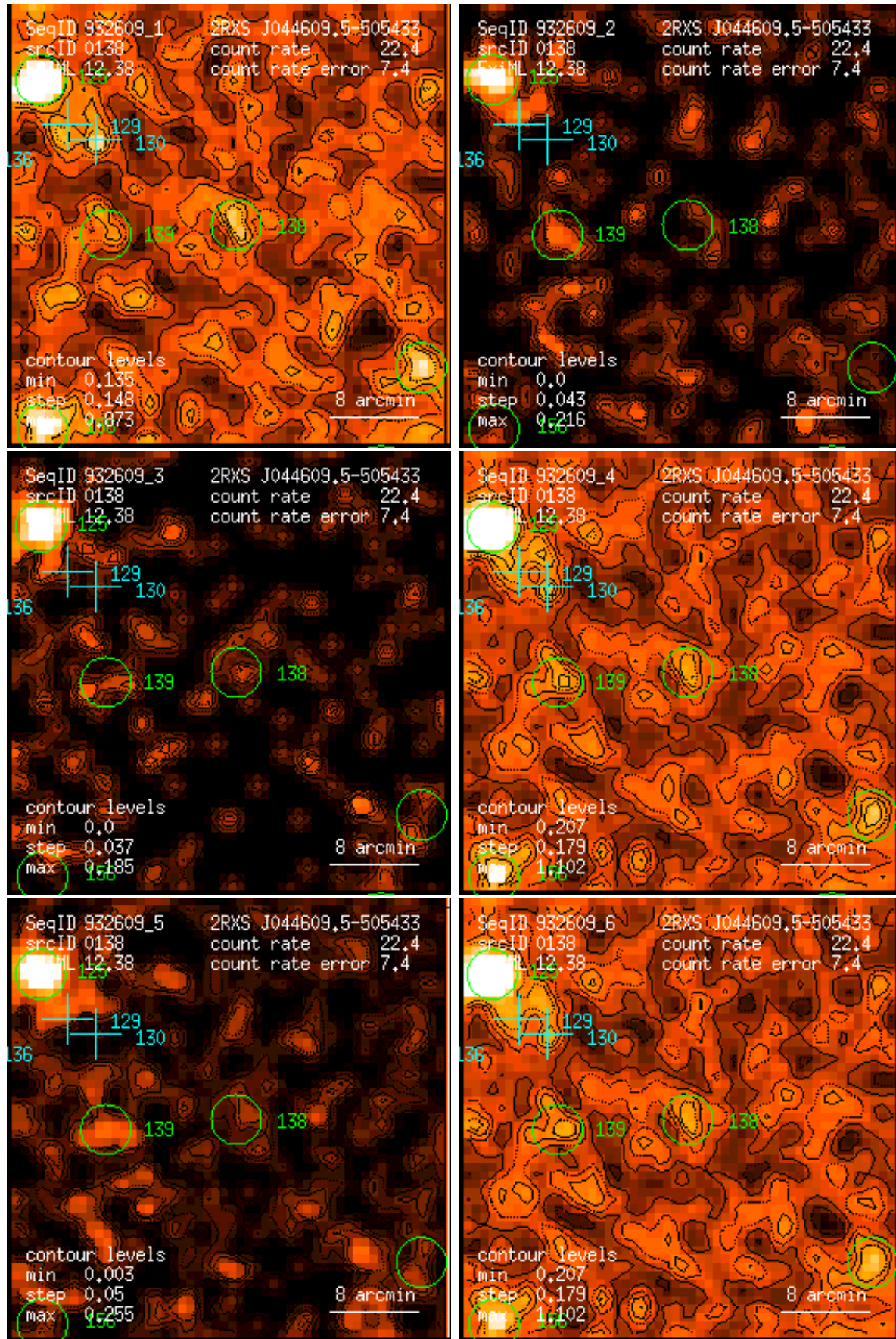
Figure 138: RASS 932609: detection 0138: band rate images, Gaussian filter: (1) PSPC channels 11 – 41, (2) 52 – 90, (3) 91 – 201, (4) 11 – 235, (5) 52 – 201, (6) 11 – 201. Broad band rates in counts/ks. Band rate contour levels in counts/ks/arcmin 2 .
