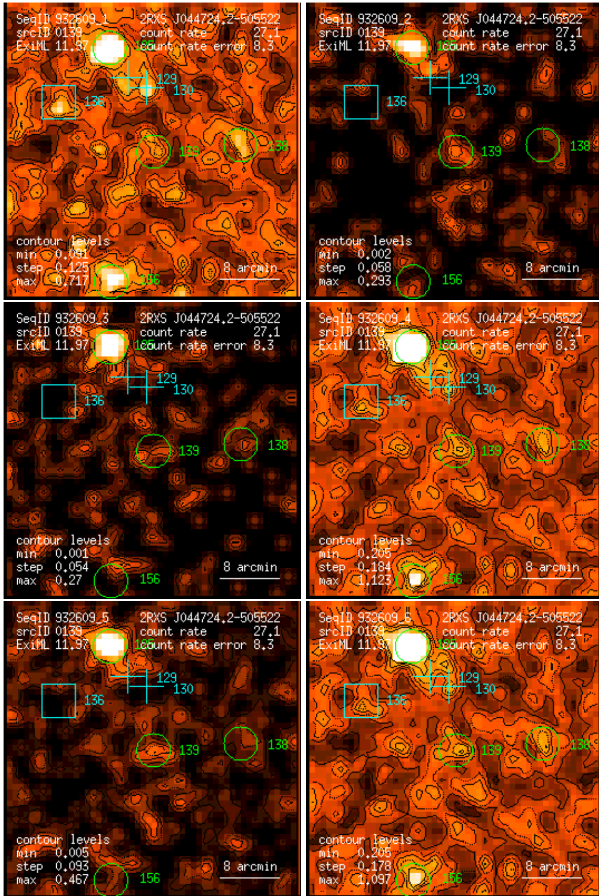
Figure 139: RASS 932609: detection 0139: band rate images, Gaussian filter: (1) PSPC channels 11 – 41, (2) 52 – 90, (3) 91 – 201, (4) 11 – 235, (5) 52 – 201, (6) 11 – 201. Broad band rates in counts/ks. Band rate contour levels in counts/ks/arcmin 2 .
