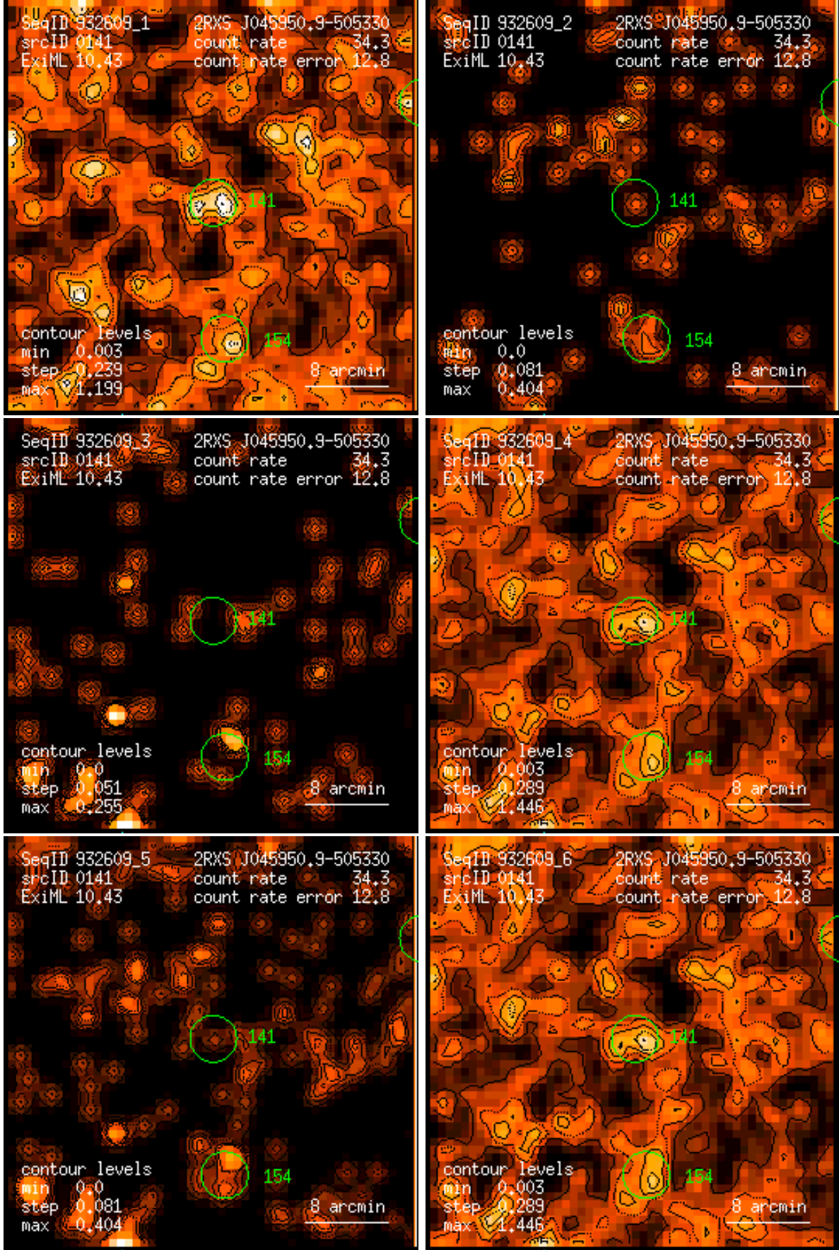
Figure 141: RASS 932609: detection 0141: band rate images, Gaussian filter: (1) PSPC channels 11 – 41, (2) 52 – 90, (3) 91 – 201, (4) 11 – 235, (5) 52 – 201, (6) 11 – 201. Broad band rates in counts/ks. Band rate contour levels in counts/ks/arcmin 2 .
