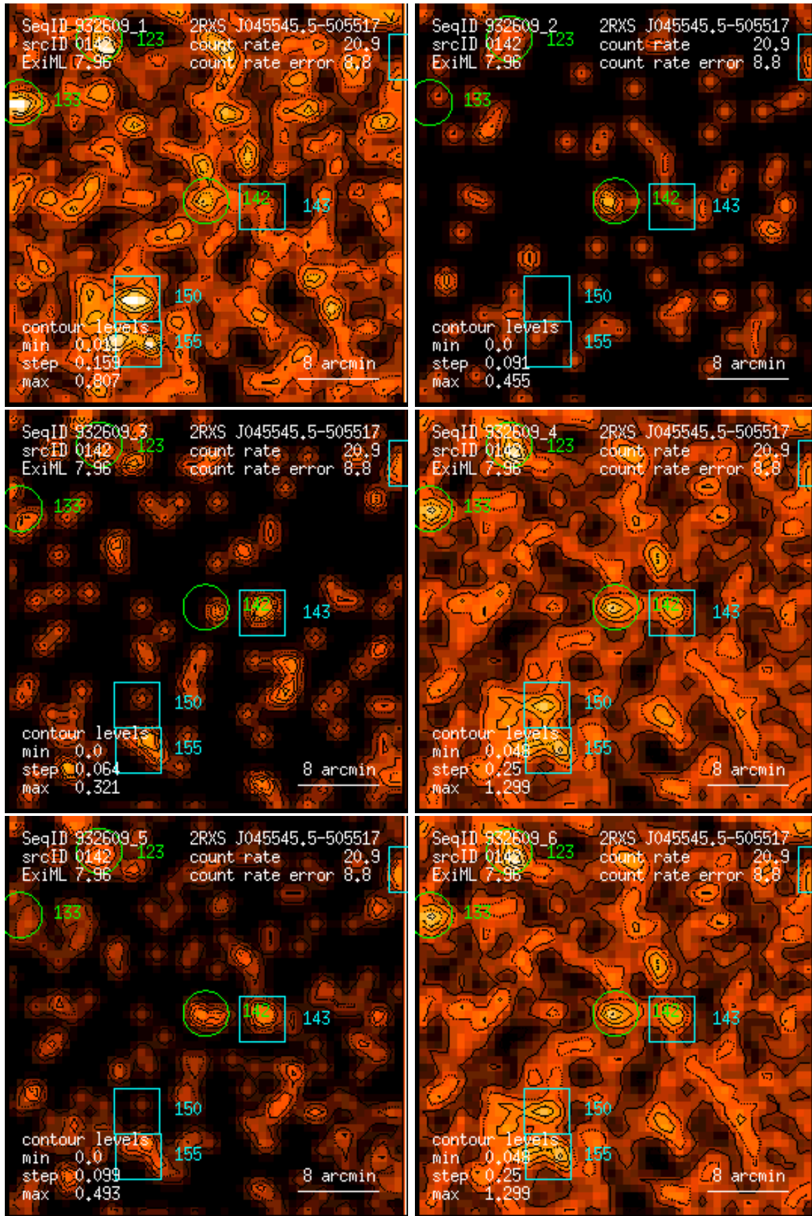
Figure 142: RASS 932609: detection 0142: band rate images, Gaussian filter: (1) PSPC channels 11 – 41, (2) 52 – 90, (3) 91 – 201, (4) 11 – 235, (5) 52 – 201, (6) 11 – 201. Broad band rates in counts/ks. Band rate contour levels in counts/ks/arcmin 2 .
