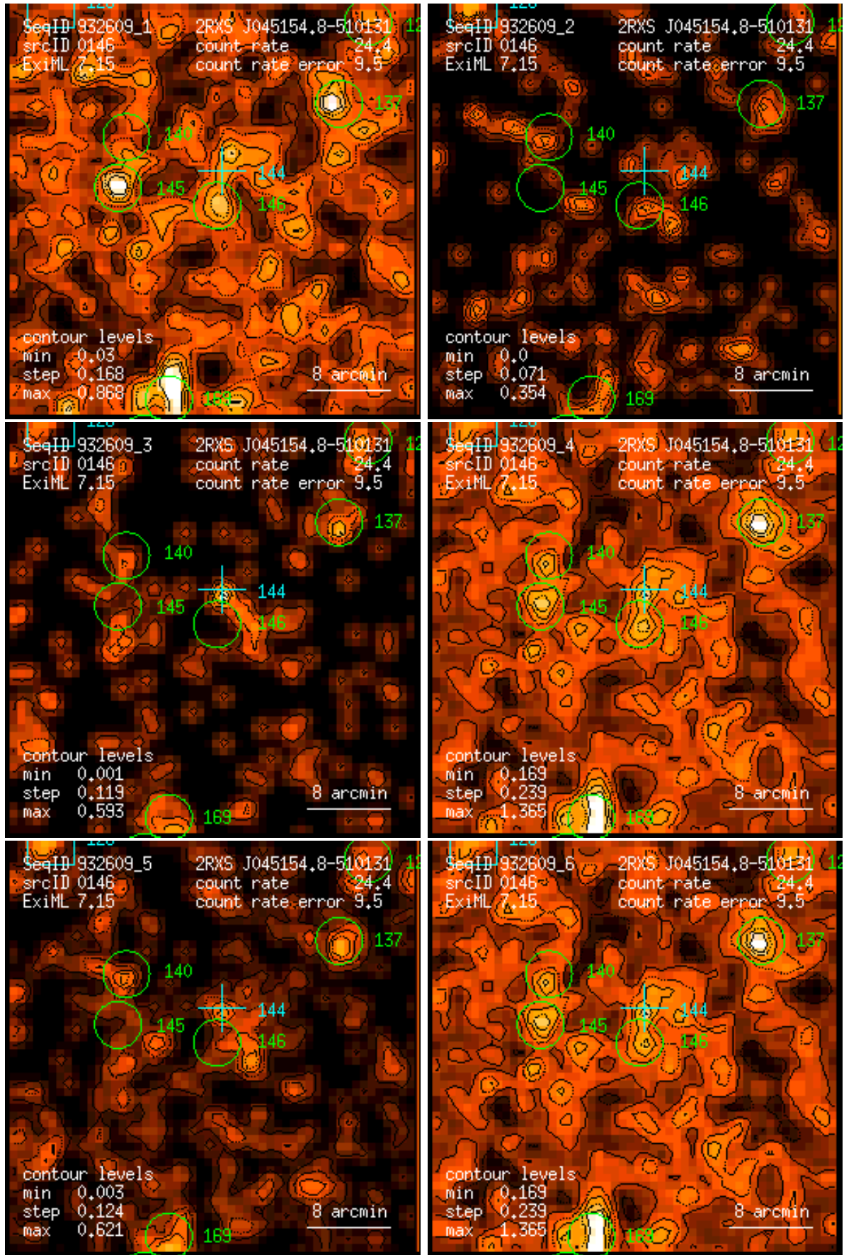
Figure 146: RASS 932609: detection 0146: band rate images, Gaussian filter: (1) PSPC channels 11 – 41, (2) 52 – 90, (3) 91 – 201, (4) 11 – 235, (5) 52 – 201, (6) 11 – 201. Broad band rates in counts/ks. Band rate contour levels in counts/ks/arcmin 2 .
