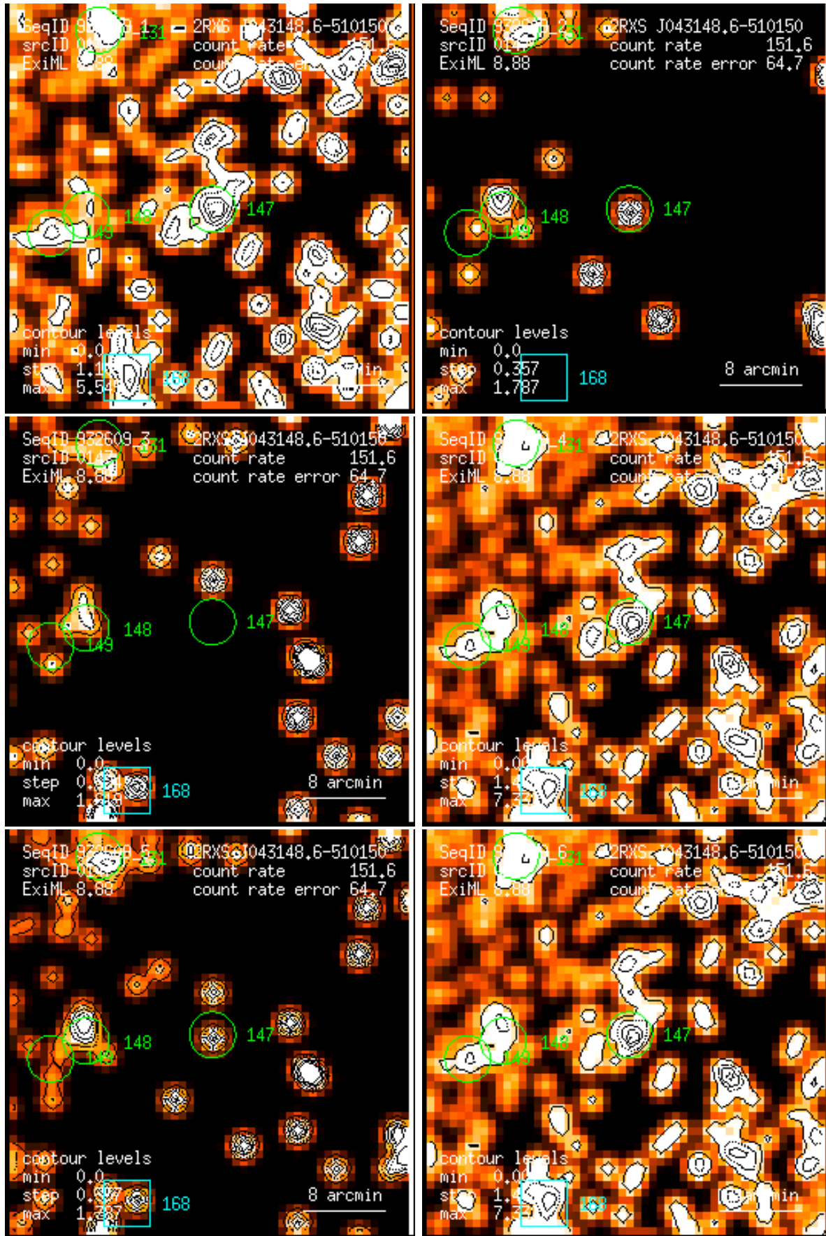
Figure 147: RASS 932609: detection 0147: band rate images, Gaussian filter: (1) PSPC channels 11 – 41, (2) 52 – 90, (3) 91 – 201, (4) 11 – 235, (5) 52 – 201, (6) 11 – 201. Broad band rates in counts/ks. Band rate contour levels in counts/ks/arcmin 2 .
