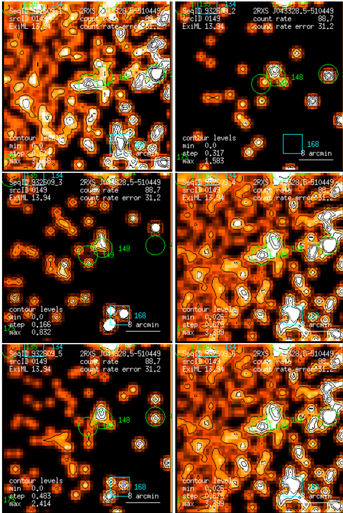
Figure 149: RASS 932609: detection 0149: band rate images, Gaussian filter: (1) PSPC channels 11 – 41, (2) 52 – 90, (3) 91 – 201, (4) 11 – 235, (5) 52 – 201, (6) 11 – 201. Broad band rates in counts/ks. Band rate contour levels in counts/ks/arcmin 2 .
