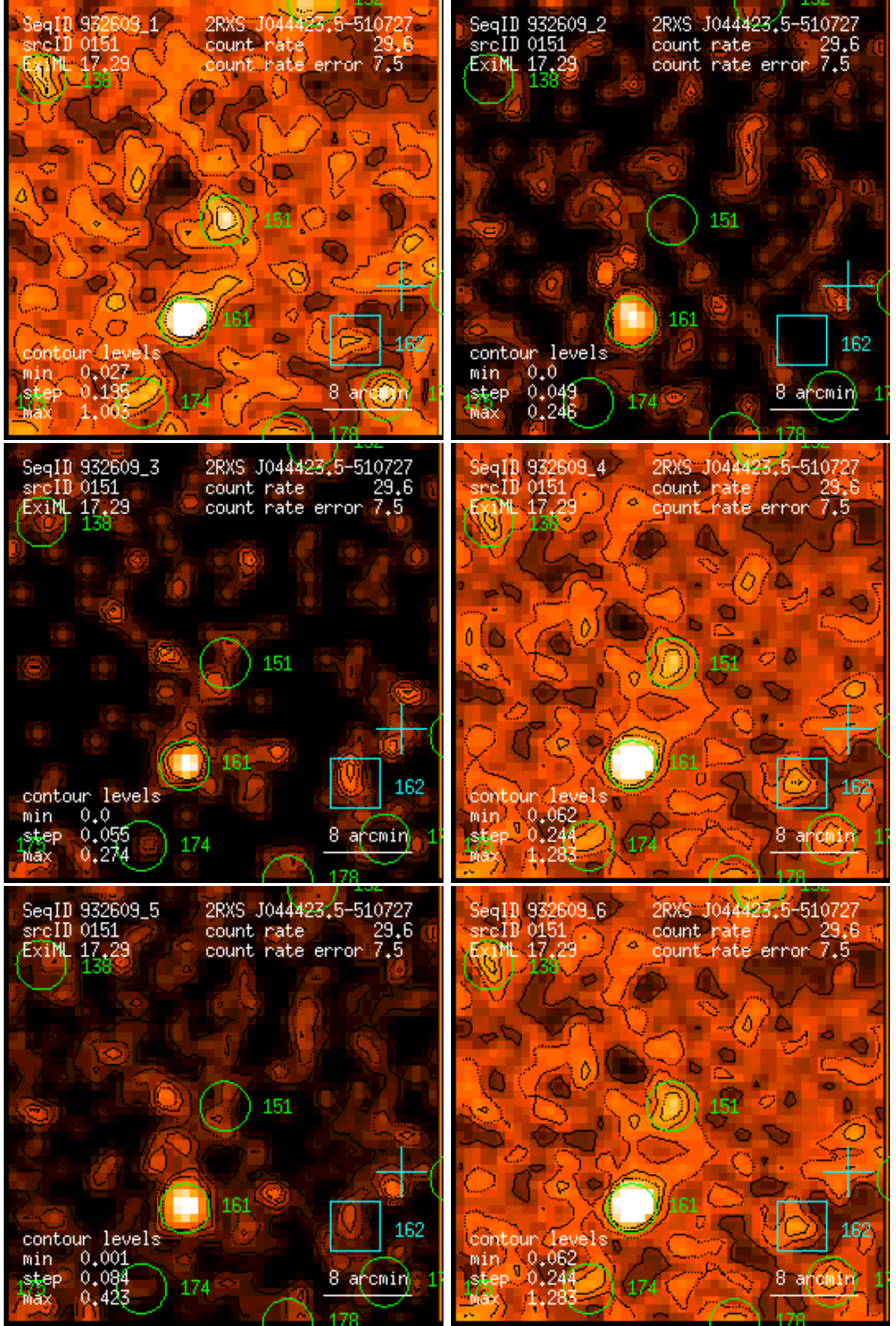
Figure 151: RASS 932609: detection 0151: band rate images, Gaussian filter: (1) PSPC channels 11 – 41, (2) 52 – 90, (3) 91 – 201, (4) 11 – 235, (5) 52 – 201, (6) 11 – 201. Broad band rates in counts/ks. Band rate contour levels in counts/ks/arcmin 2 .
