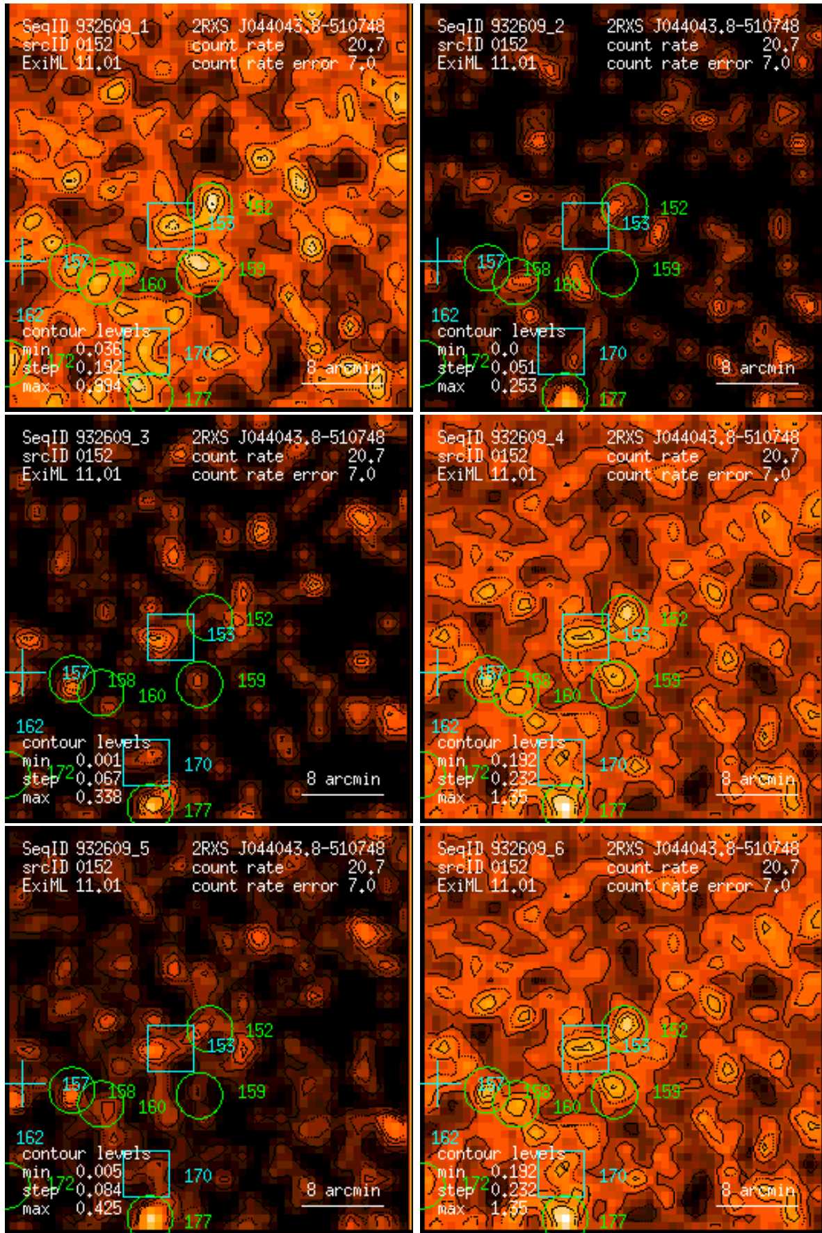
Figure 152: RASS 932609: detection 0152: band rate images, Gaussian filter: (1) PSPC channels 11 – 41, (2) 52 – 90, (3) 91 – 201, (4) 11 – 235, (5) 52 – 201, (6) 11 – 201. Broad band rates in counts/ks. Band rate contour levels in counts/ks/arcmin 2 .
