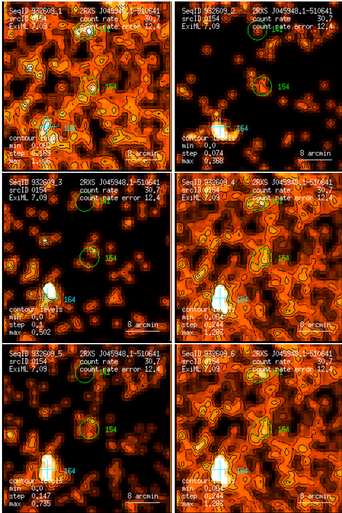
Figure 154: RASS 932609: detection 0154: band rate images, Gaussian filter: (1) PSPC channels 11 – 41, (2) 52 – 90, (3) 91 – 201, (4) 11 – 235, (5) 52 – 201, (6) 11 – 201. Broad band rates in counts/ks. Band rate contour levels in counts/ks/arcmin 2 .
