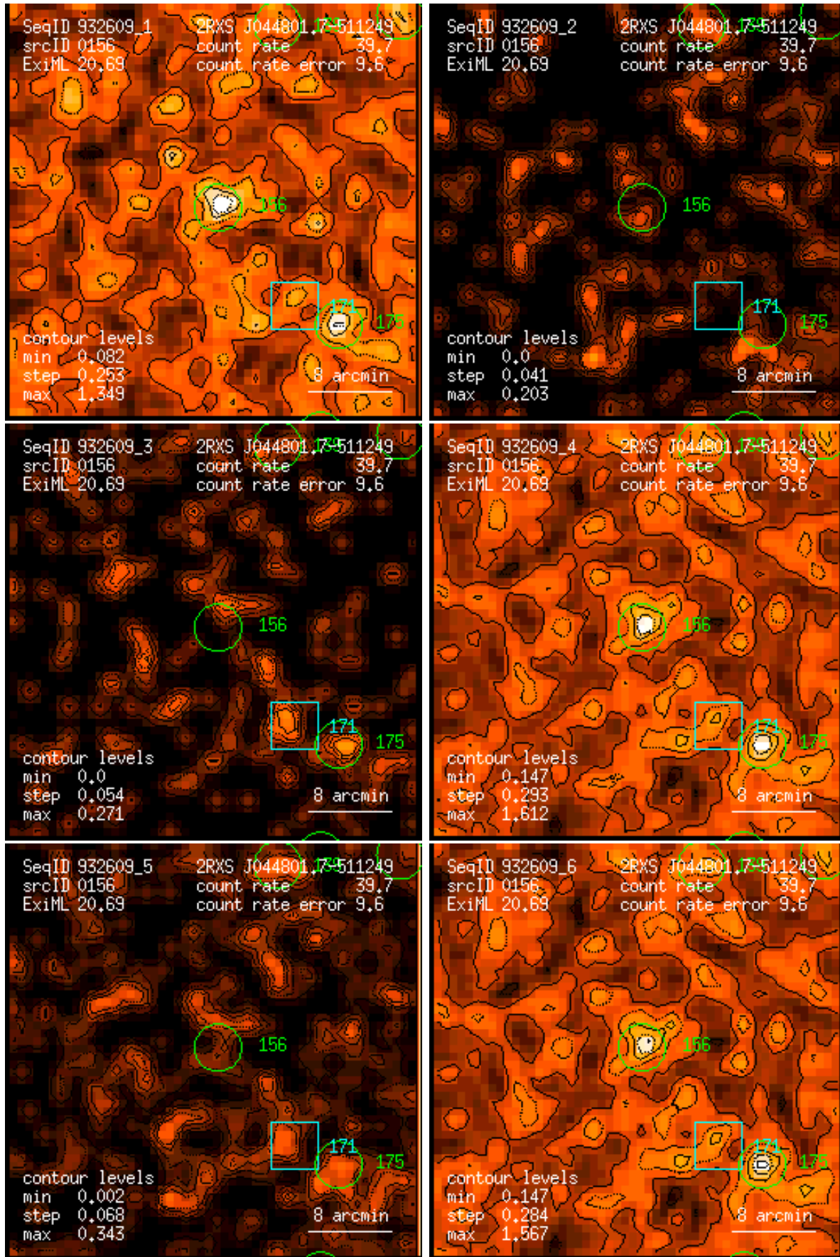
Figure 156: RASS 932609: detection 0156: band rate images, Gaussian filter: (1) PSPC channels 11 – 41, (2) 52 – 90, (3) 91 – 201, (4) 11 – 235, (5) 52 – 201, (6) 11 – 201. Broad band rates in counts/ks. Band rate contour levels in counts/ks/arcmin 2 .
