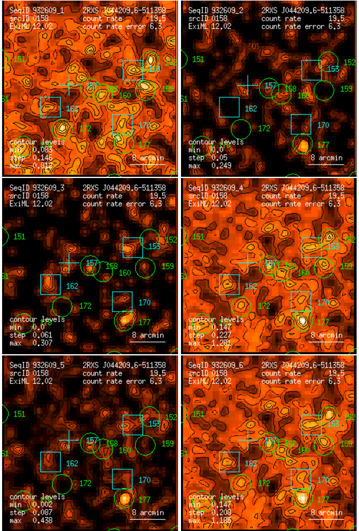
Figure 158: RASS 932609: detection 0158: band rate images, Gaussian filter: (1) PSPC channels 11 – 41, (2) 52 – 90, (3) 91 – 201, (4) 11 – 235, (5) 52 – 201, (6) 11 – 201. Broad band rates in counts/ks. Band rate contour levels in counts/ks/arcmin 2 .
