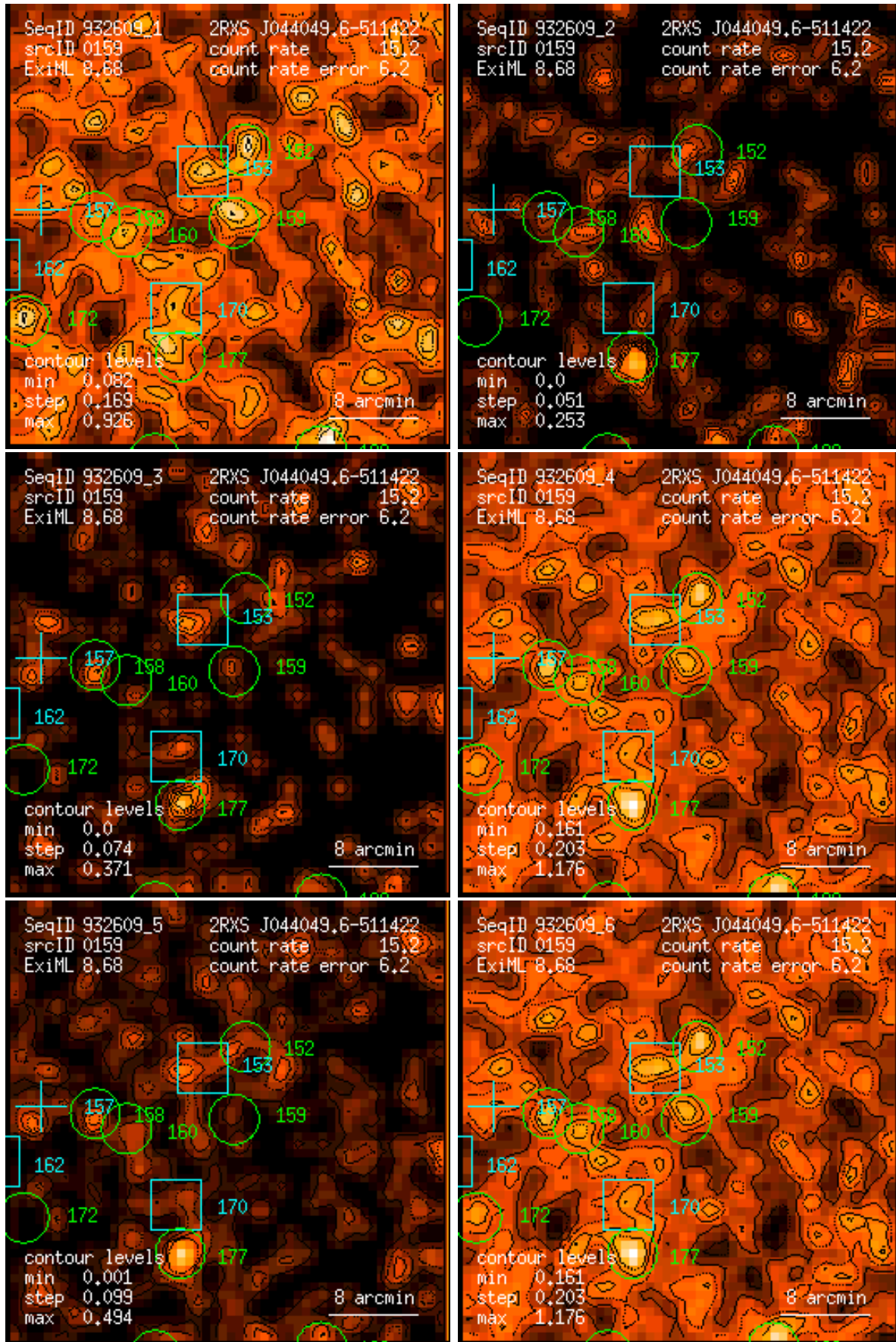
Figure 159: RASS 932609: detection 0159: band rate images, Gaussian filter: (1) PSPC channels 11 – 41, (2) 52 – 90, (3) 91 – 201, (4) 11 – 235, (5) 52 – 201, (6) 11 – 201. Broad band rates in counts/ks. Band rate contour levels in counts/ks/arcmin 2 .
