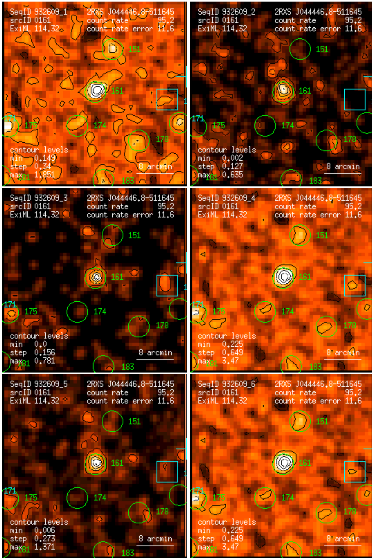
Figure 161: RASS 932609: detection 0161: band rate images, Gaussian filter: (1) PSPC channels 11 – 41, (2) 52 – 90, (3) 91 – 201, (4) 11 – 235, (5) 52 – 201, (6) 11 – 201. Broad band rates in counts/ks. Band rate contour levels in counts/ks/arcmin 2 .
