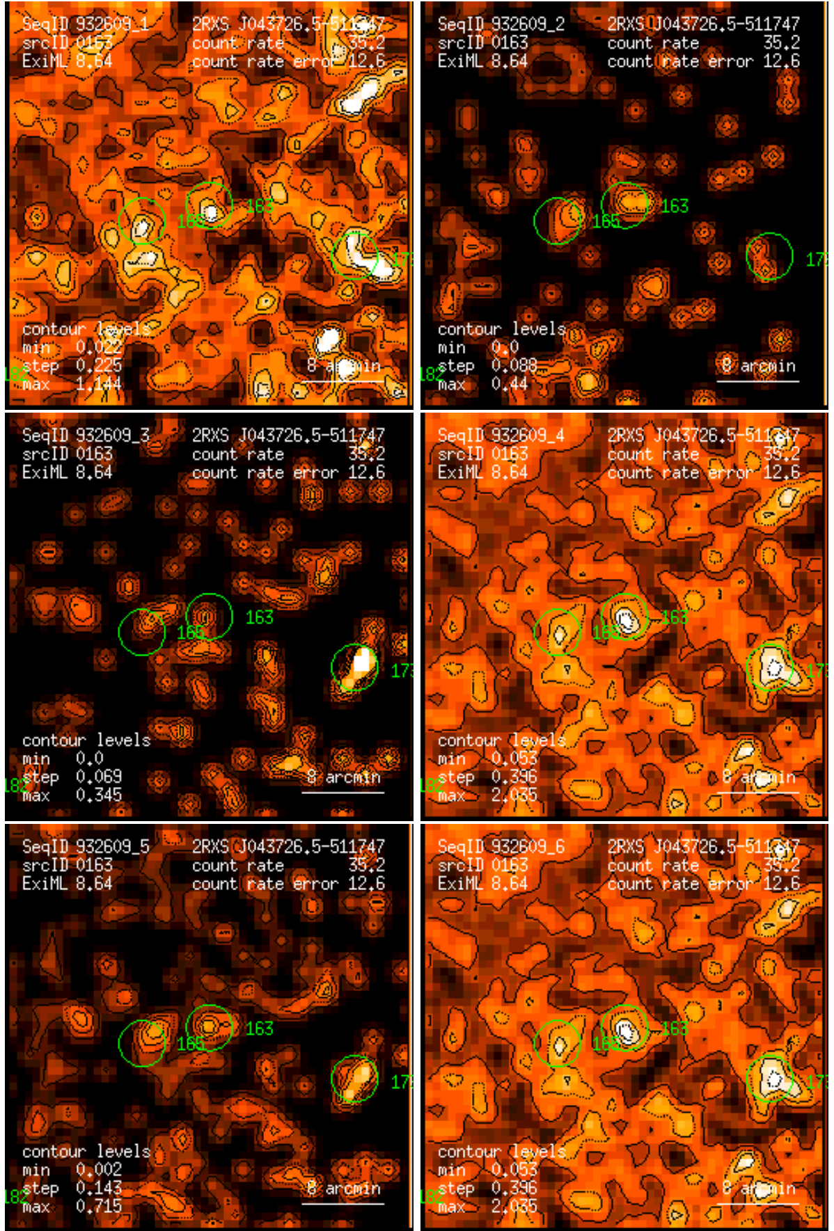
Figure 163: RASS 932609: detection 0163: band rate images, Gaussian filter: (1) PSPC channels 11 – 41, (2) 52 – 90, (3) 91 – 201, (4) 11 – 235, (5) 52 – 201, (6) 11 – 201. Broad band rates in counts/ks. Band rate contour levels in counts/ks/arcmin 2 .
