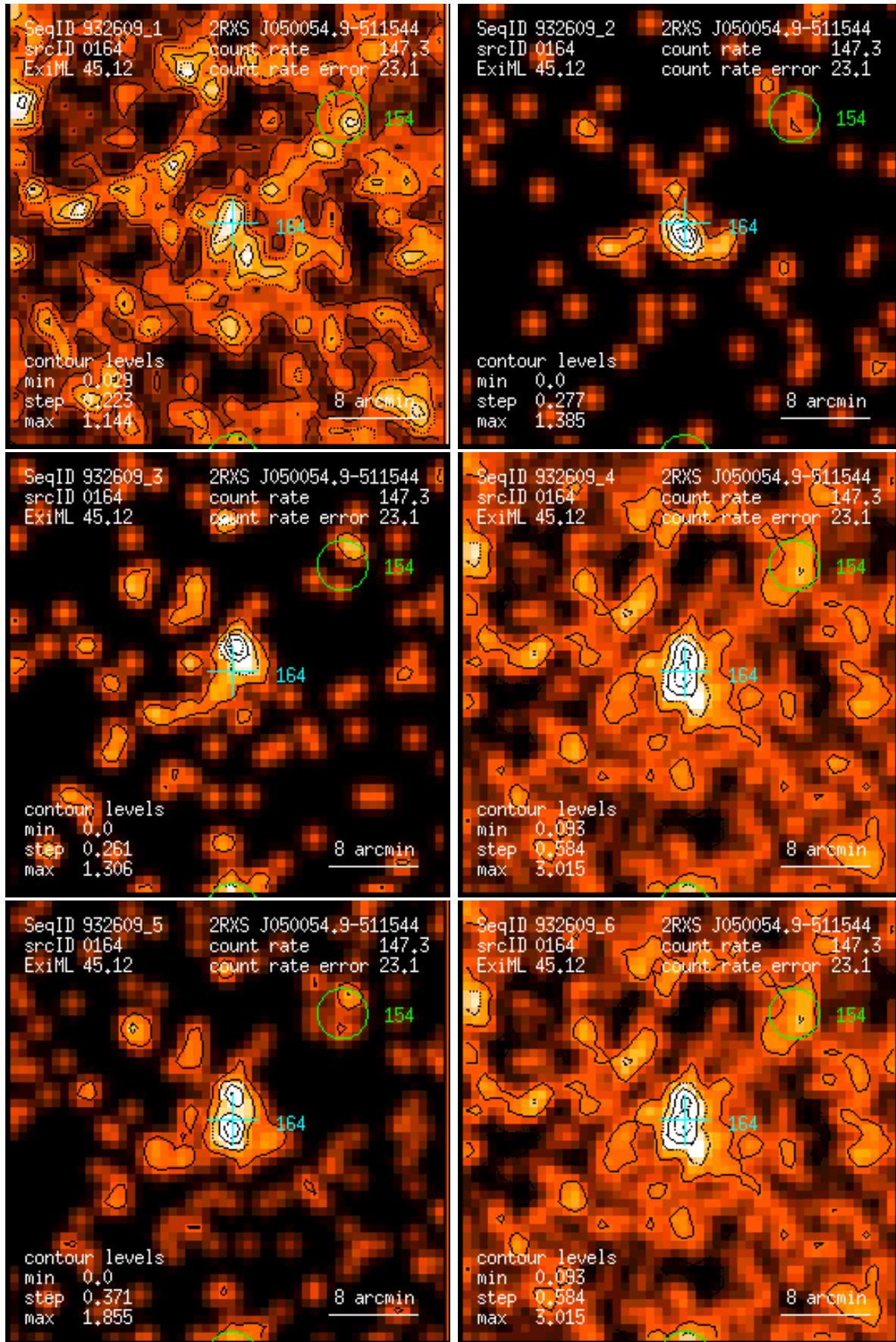
Figure 164: RASS 932609: detection 0164: band rate images, Gaussian filter: (1) PSPC channels 11 – 41, (2) 52 – 90, (3) 91 – 201, (4) 11 – 235, (5) 52 – 201, (6) 11 – 201. Broad band rates in counts/ks. Band rate contour levels in counts/ks/arcmin 2 .
