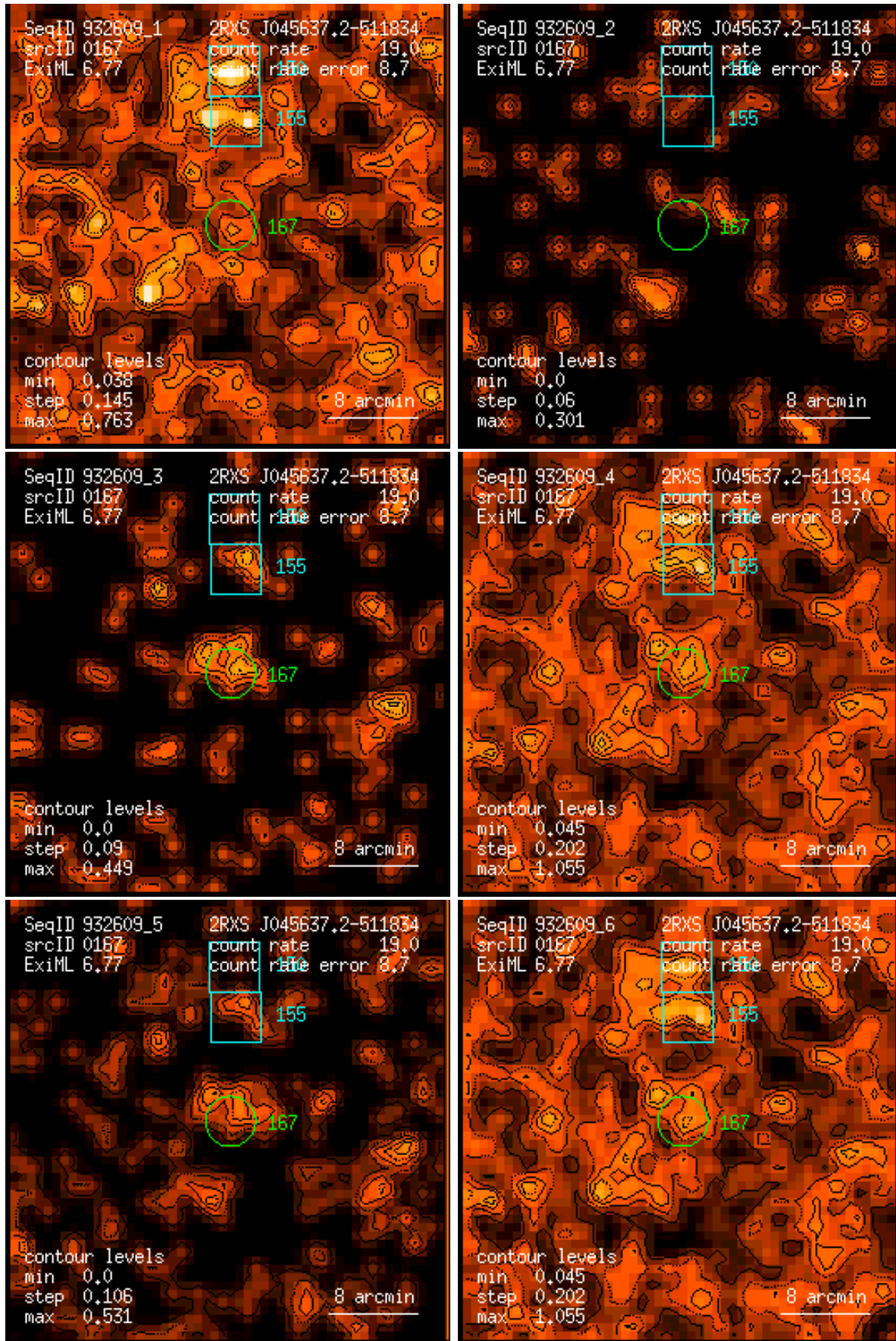
Figure 167: RASS 932609: detection 0167: band rate images, Gaussian filter: (1) PSPC channels 11 – 41, (2) 52 – 90, (3) 91 – 201, (4) 11 – 235, (5) 52 – 201, (6) 11 – 201. Broad band rates in counts/ks. Band rate contour levels in counts/ks/arcmin 2 .
