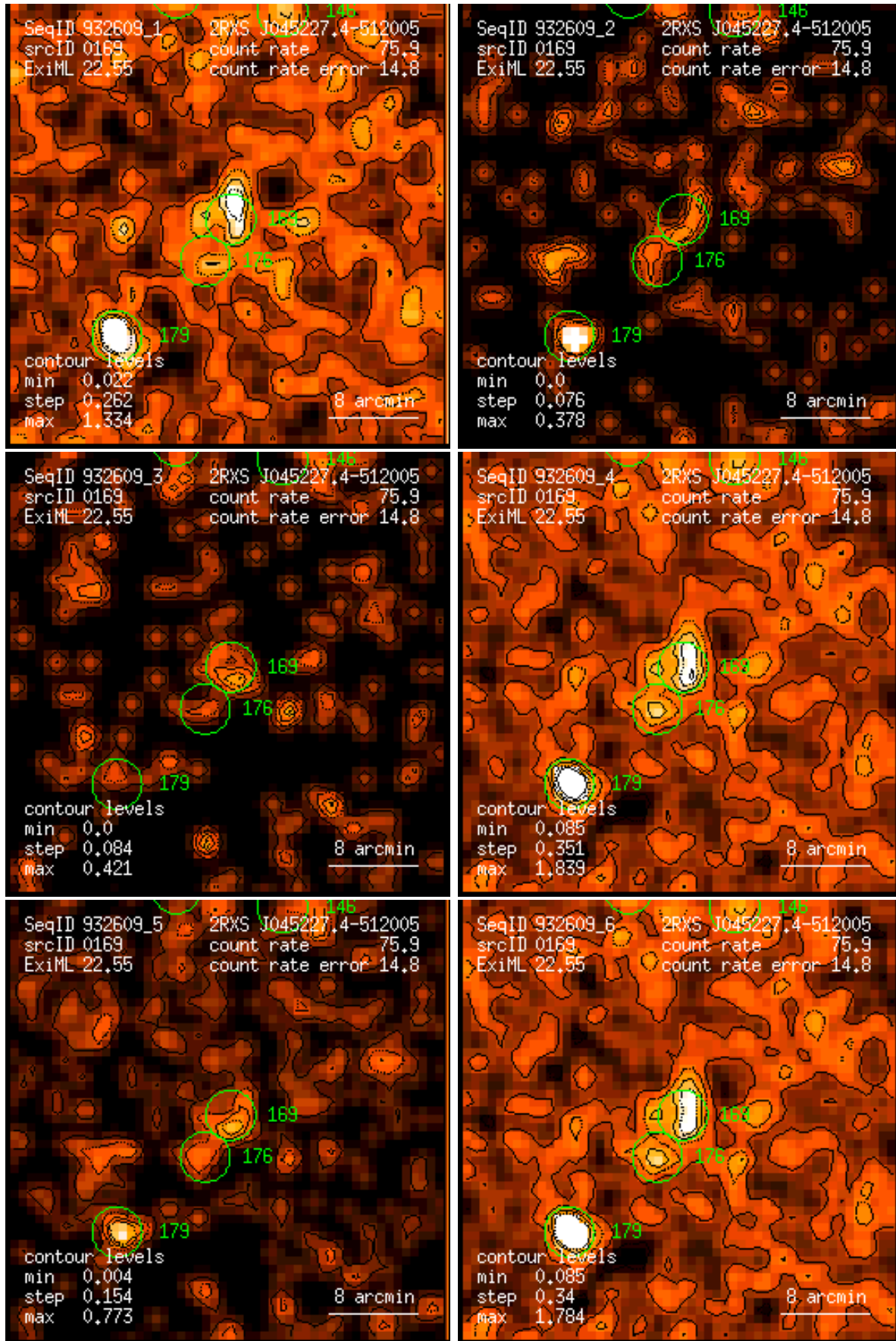
Figure 169: RASS 932609: detection 0169: band rate images, Gaussian filter: (1) PSPC channels 11 – 41, (2) 52 – 90, (3) 91 – 201, (4) 11 – 235, (5) 52 – 201, (6) 11 – 201. Broad band rates in counts/ks. Band rate contour levels in counts/ks/arcmin 2 .
