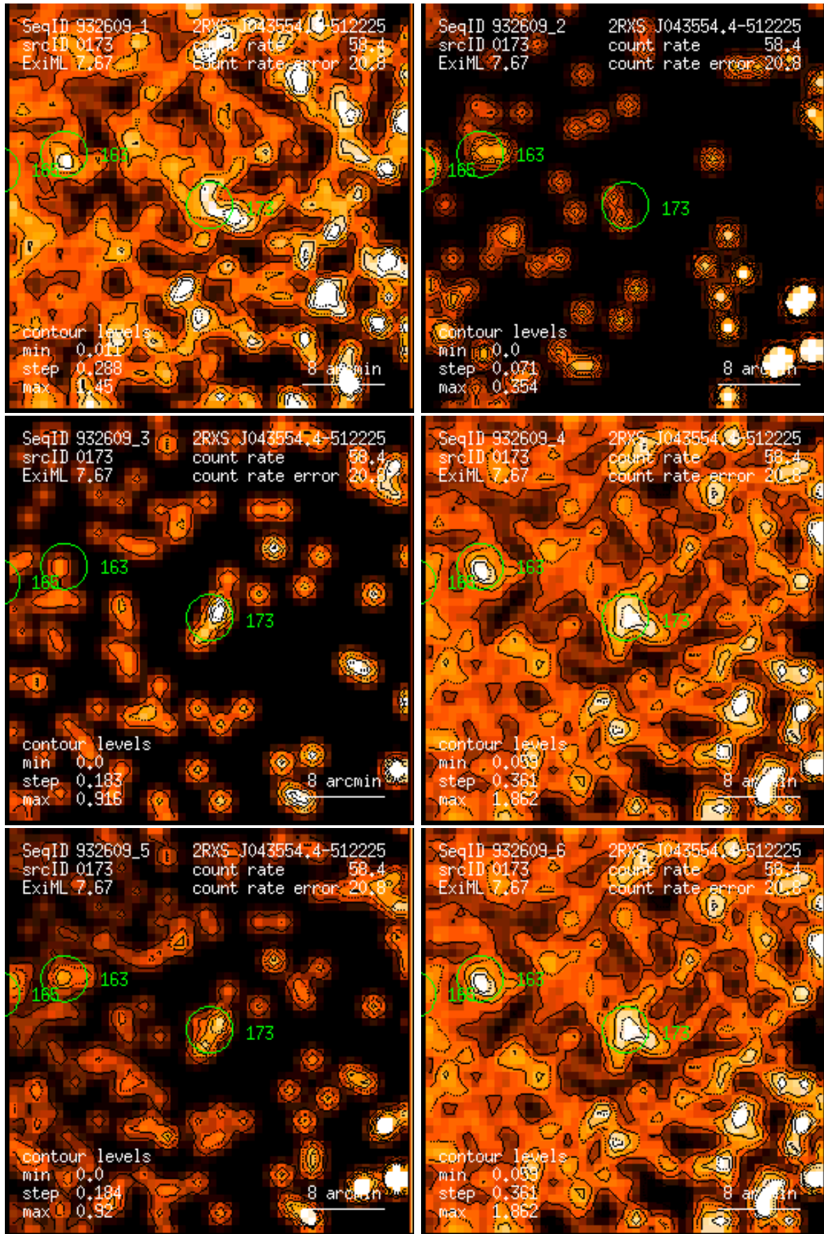
Figure 173: RASS 932609: detection 0173: band rate images, Gaussian filter: (1) PSPC channels 11 – 41, (2) 52 – 90, (3) 91 – 201, (4) 11 – 235, (5) 52 – 201, (6) 11 – 201. Broad band rates in counts/ks. Band rate contour levels in counts/ks/arcmin 2 .
