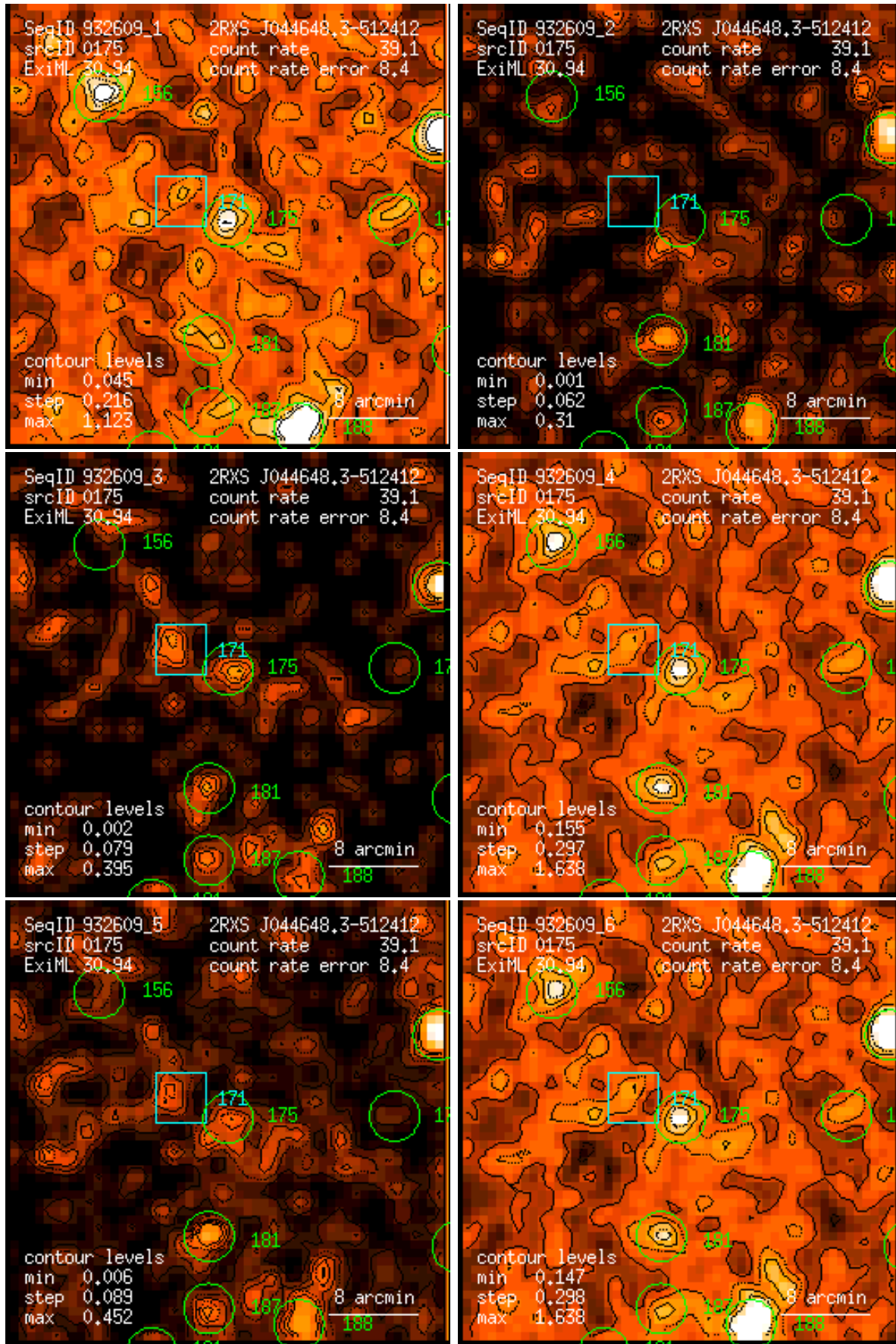
Figure 175: RASS 932609: detection 0175: band rate images, Gaussian filter: (1) PSPC channels 11 – 41, (2) 52 – 90, (3) 91 – 201, (4) 11 – 235, (5) 52 – 201, (6) 11 – 201. Broad band rates in counts/ks. Band rate contour levels in counts/ks/arcmin 2 .
