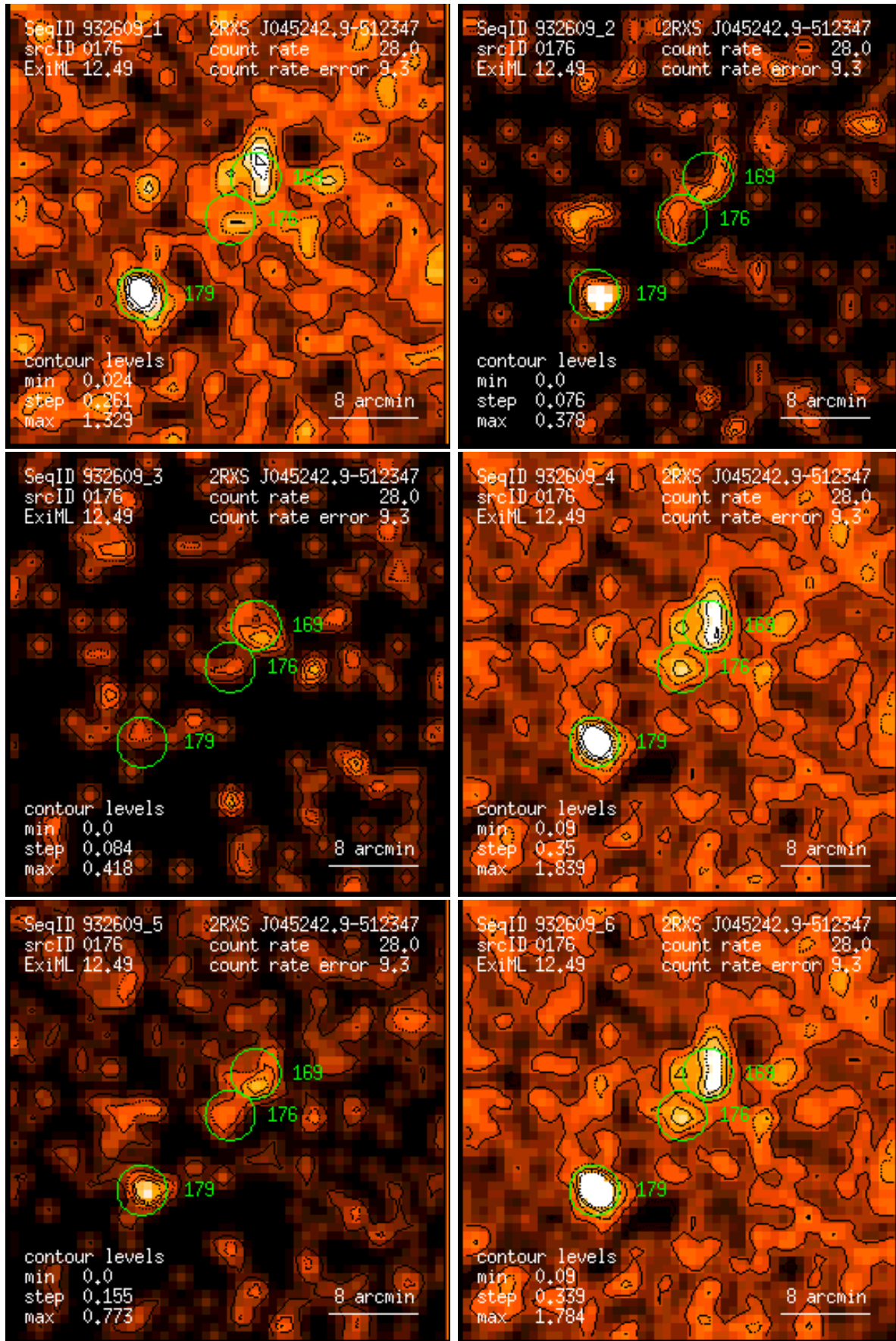
Figure 176: RASS 932609: detection 0176: band rate images, Gaussian filter: (1) PSPC channels 11 – 41, (2) 52 – 90, (3) 91 – 201, (4) 11 – 235, (5) 52 – 201, (6) 11 – 201. Broad band rates in counts/ks. Band rate contour levels in counts/ks/arcmin 2 .
