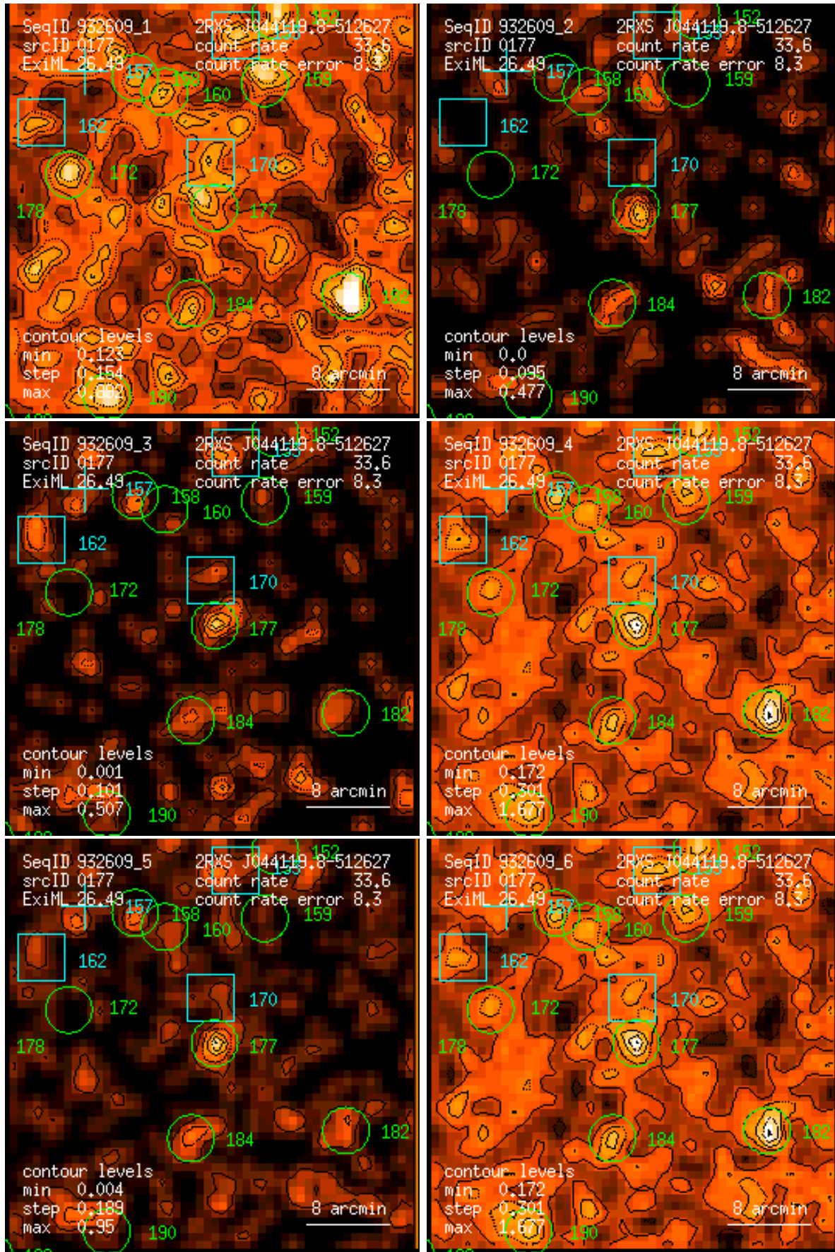
Figure 177: RASS 932609: detection 0177: band rate images, Gaussian filter: (1) PSPC channels 11 – 41, (2) 52 – 90, (3) 91 – 201, (4) 11 – 235, (5) 52 – 201, (6) 11 – 201. Broad band rates in counts/ks. Band rate contour levels in counts/ks/arcmin 2 .
