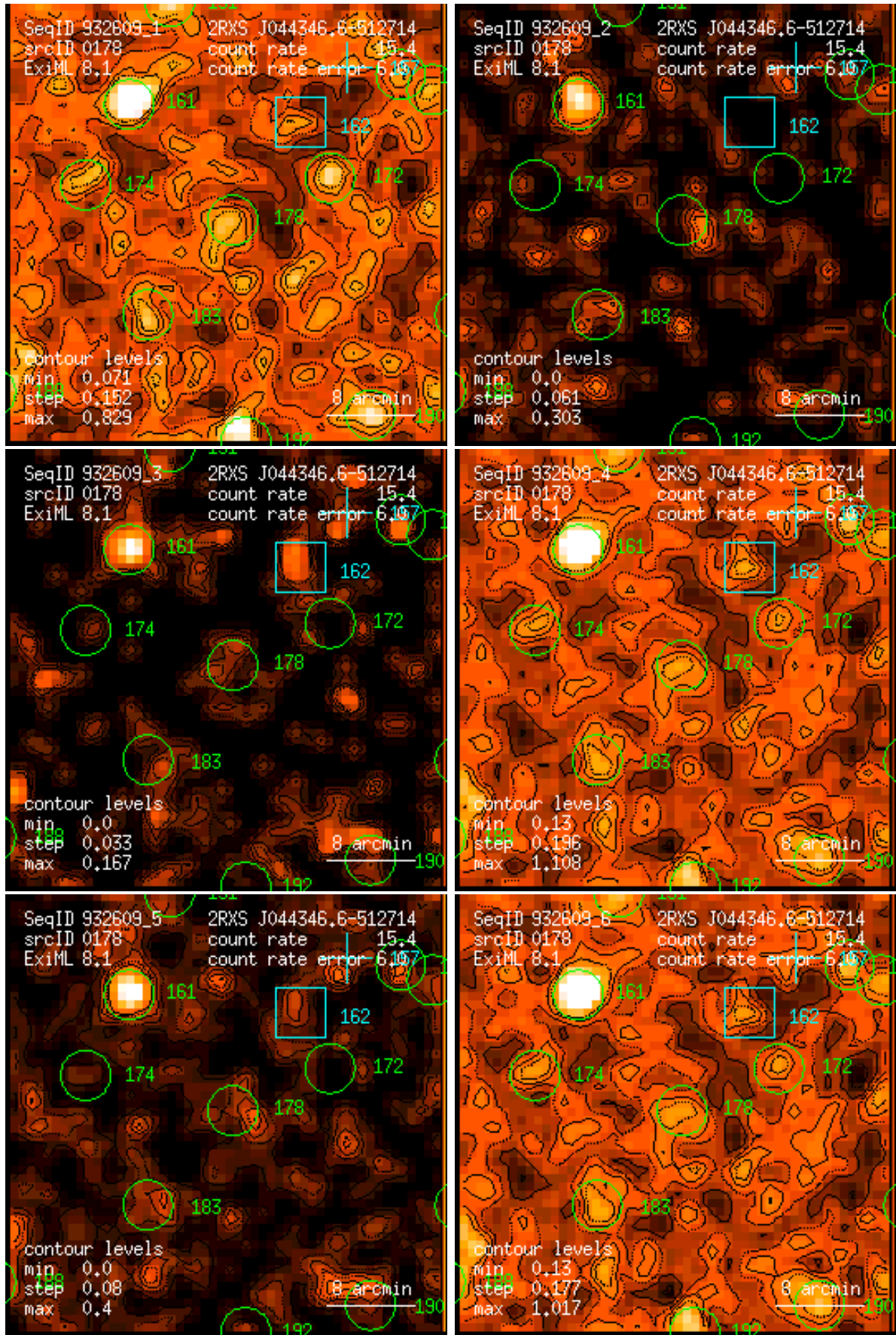
Figure 178: RASS 932609: detection 0178: band rate images, Gaussian filter: (1) PSPC channels 11 – 41, (2) 52 – 90, (3) 91 – 201, (4) 11 – 235, (5) 52 – 201, (6) 11 – 201. Broad band rates in counts/ks. Band rate contour levels in counts/ks/arcmin 2 .
