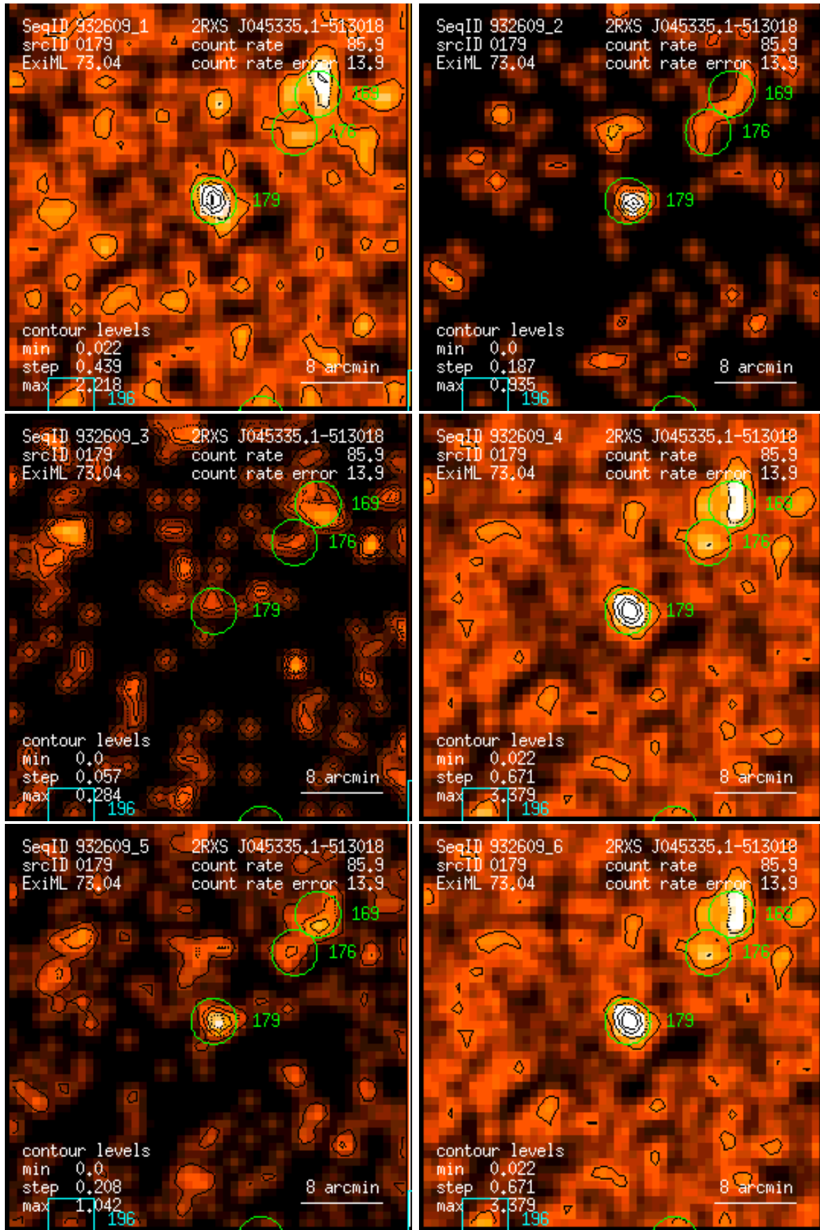
Figure 179: RASS 932609: detection 0179: band rate images, Gaussian filter: (1) PSPC channels 11 – 41, (2) 52 – 90, (3) 91 – 201, (4) 11 – 235, (5) 52 – 201, (6) 11 – 201. Broad band rates in counts/ks. Band rate contour levels in counts/ks/arcmin 2 .
