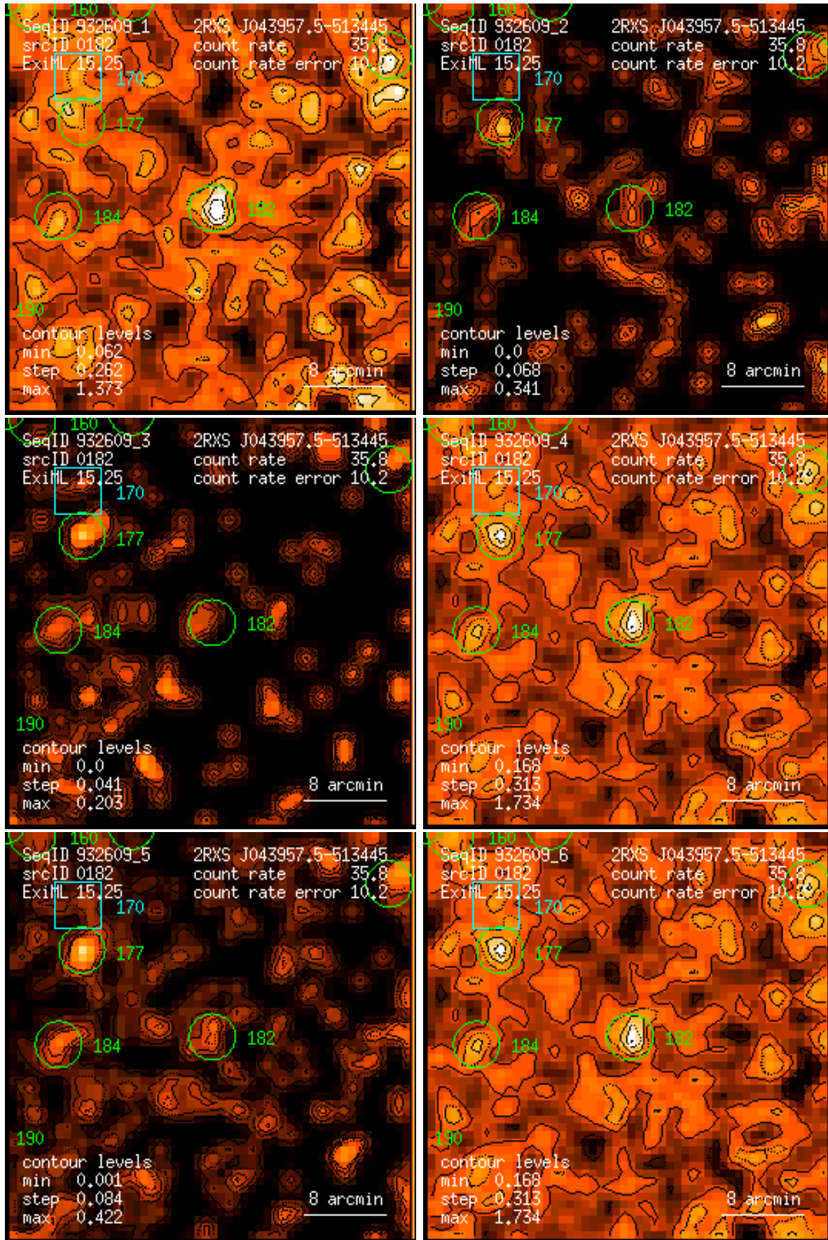
Figure 182: RASS 932609: detection 0182: band rate images, Gaussian filter: (1) PSPC channels 11 – 41, (2) 52 – 90, (3) 91 – 201, (4) 11 – 235, (5) 52 – 201, (6) 11 – 201. Broad band rates in counts/ks. Band rate contour levels in counts/ks/arcmin 2 .
