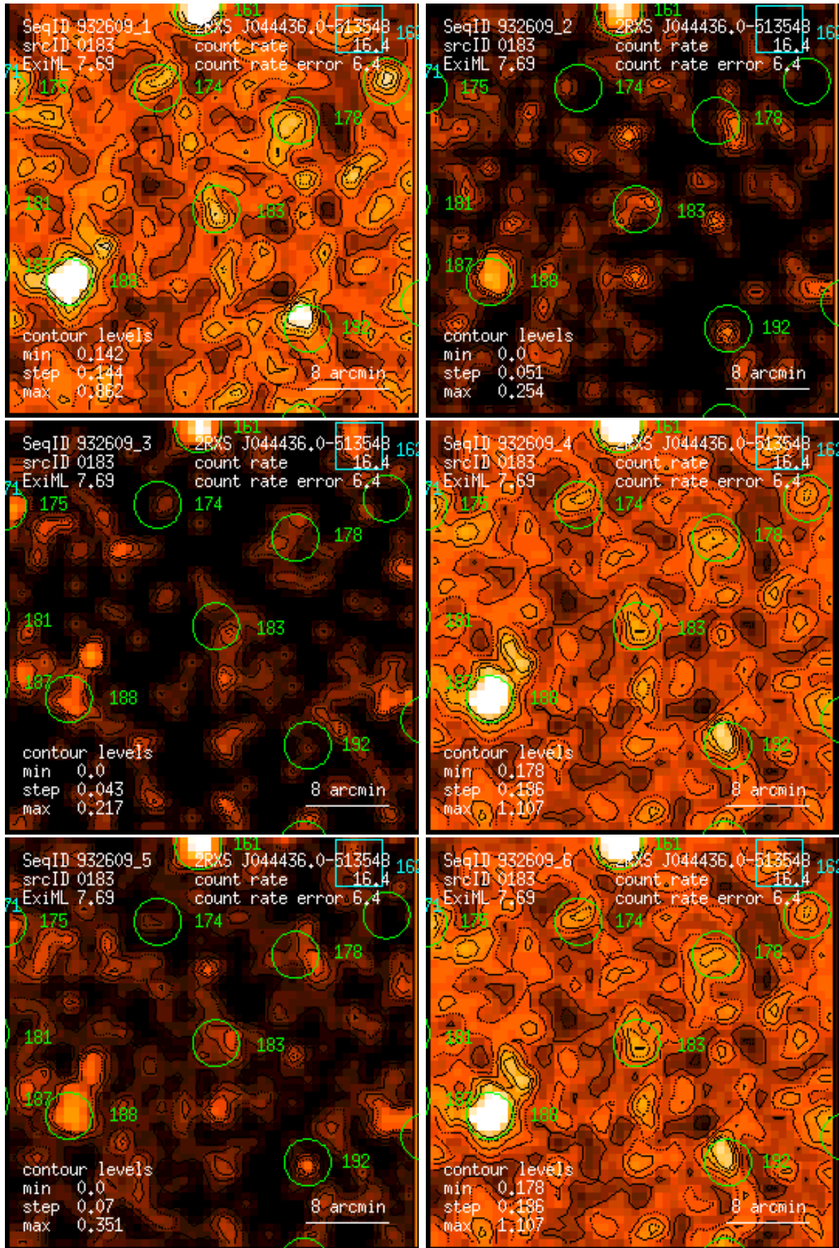
Figure 183: RASS 932609: detection 0183: band rate images, Gaussian filter: (1) PSPC channels 11 – 41, (2) 52 – 90, (3) 91 – 201, (4) 11 – 235, (5) 52 – 201, (6) 11 – 201. Broad band rates in counts/ks. Band rate contour levels in counts/ks/arcmin 2 .
