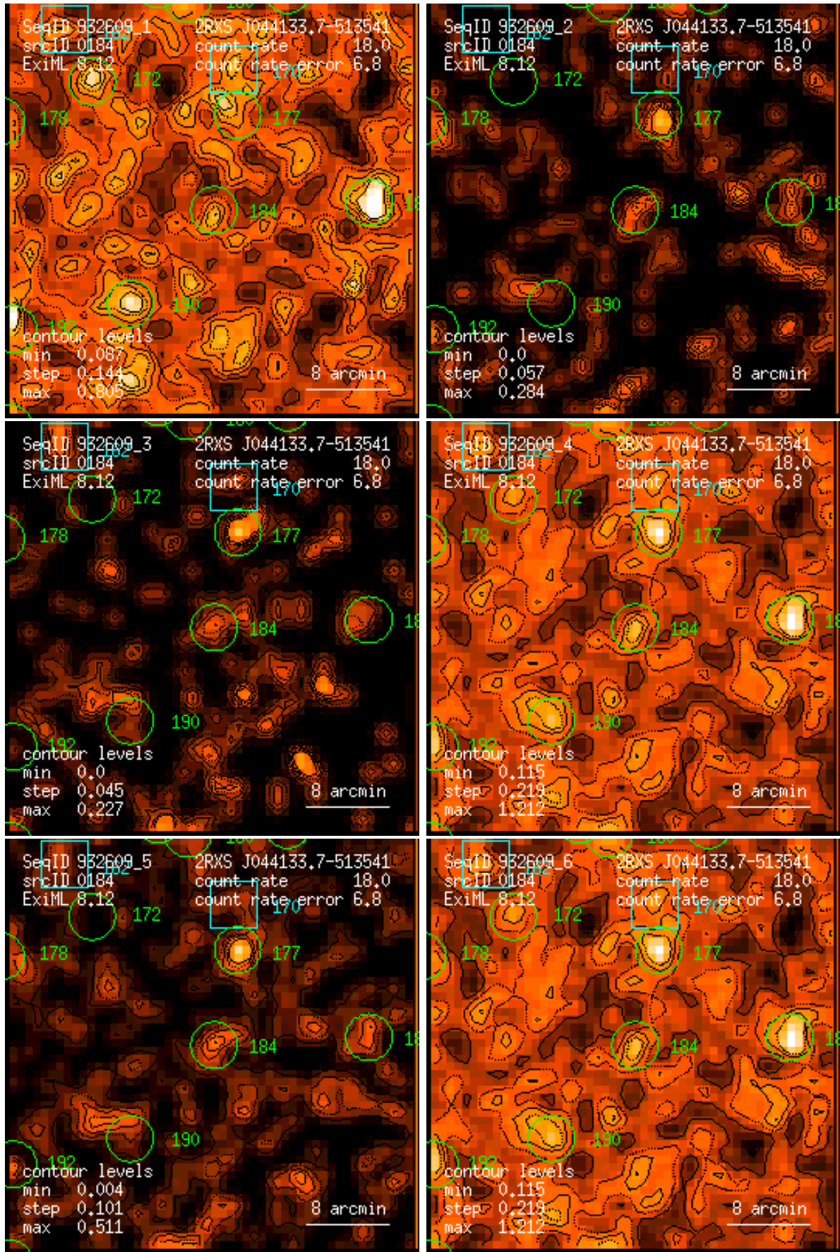
Figure 184: RASS 932609: detection 0184: band rate images, Gaussian filter: (1) PSPC channels 11 – 41, (2) 52 – 90, (3) 91 – 201, (4) 11 – 235, (5) 52 – 201, (6) 11 – 201. Broad band rates in counts/ks. Band rate contour levels in counts/ks/arcmin 2 .
