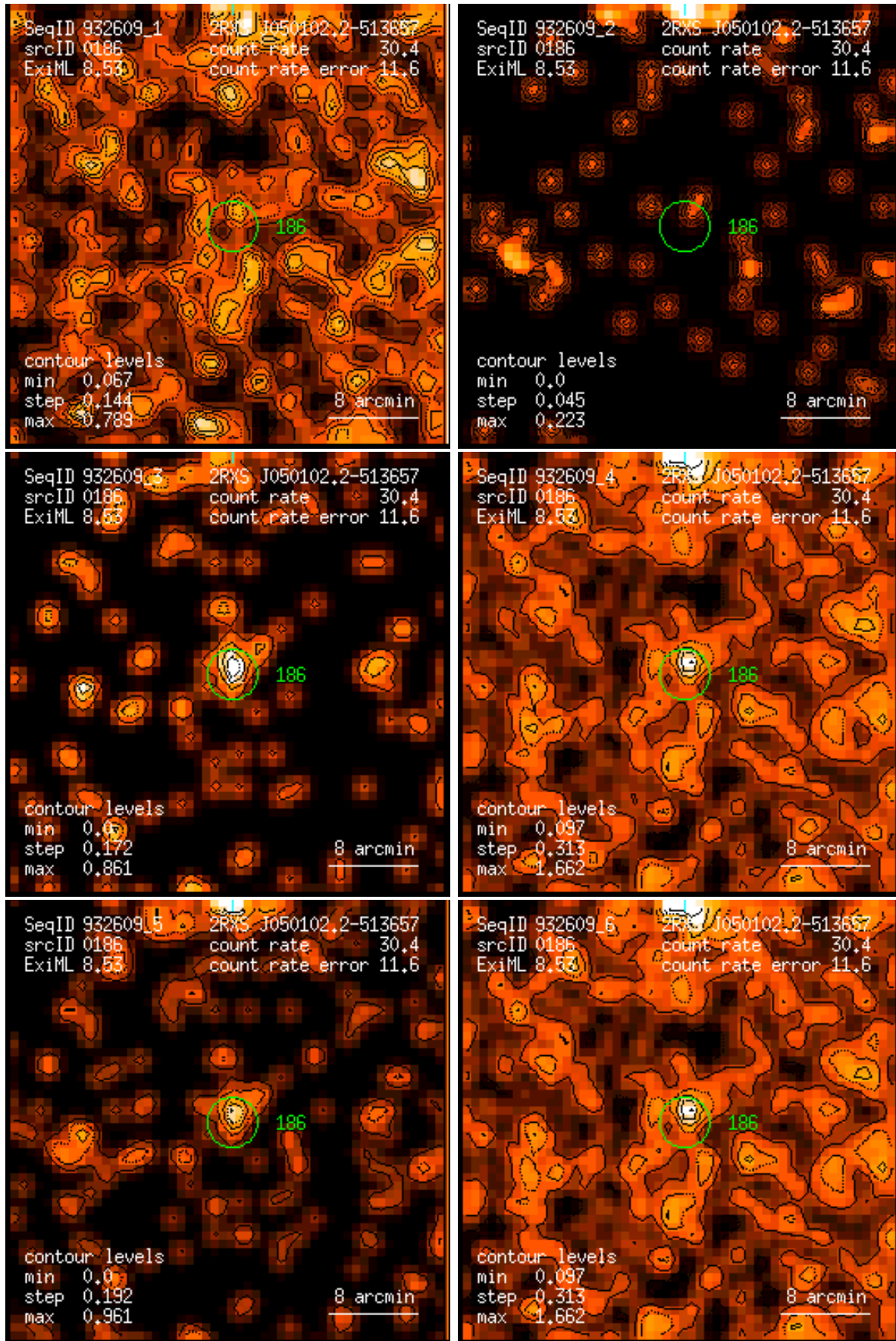
Figure 186: RASS 932609: detection 0186: band rate images, Gaussian filter: (1) PSPC channels 11 – 41, (2) 52 – 90, (3) 91 – 201, (4) 11 – 235, (5) 52 – 201, (6) 11 – 201. Broad band rates in counts/ks. Band rate contour levels in counts/ks/arcmin 2 .
