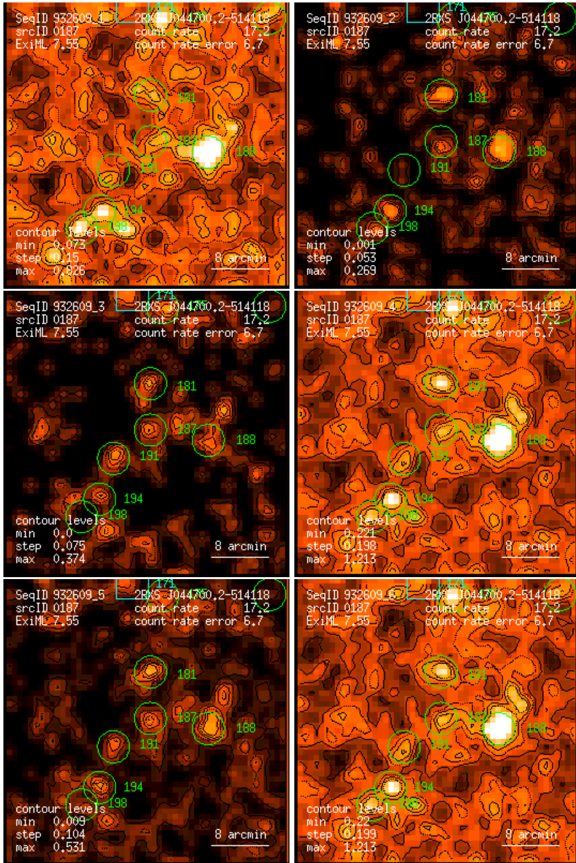
Figure 187: RASS 932609: detection 0187: band rate images, Gaussian filter: (1) PSPC channels 11 – 41, (2) 52 – 90, (3) 91 – 201, (4) 11 – 235, (5) 52 – 201, (6) 11 – 201. Broad band rates in counts/ks. Band rate contour levels in counts/ks/arcmin 2 .
