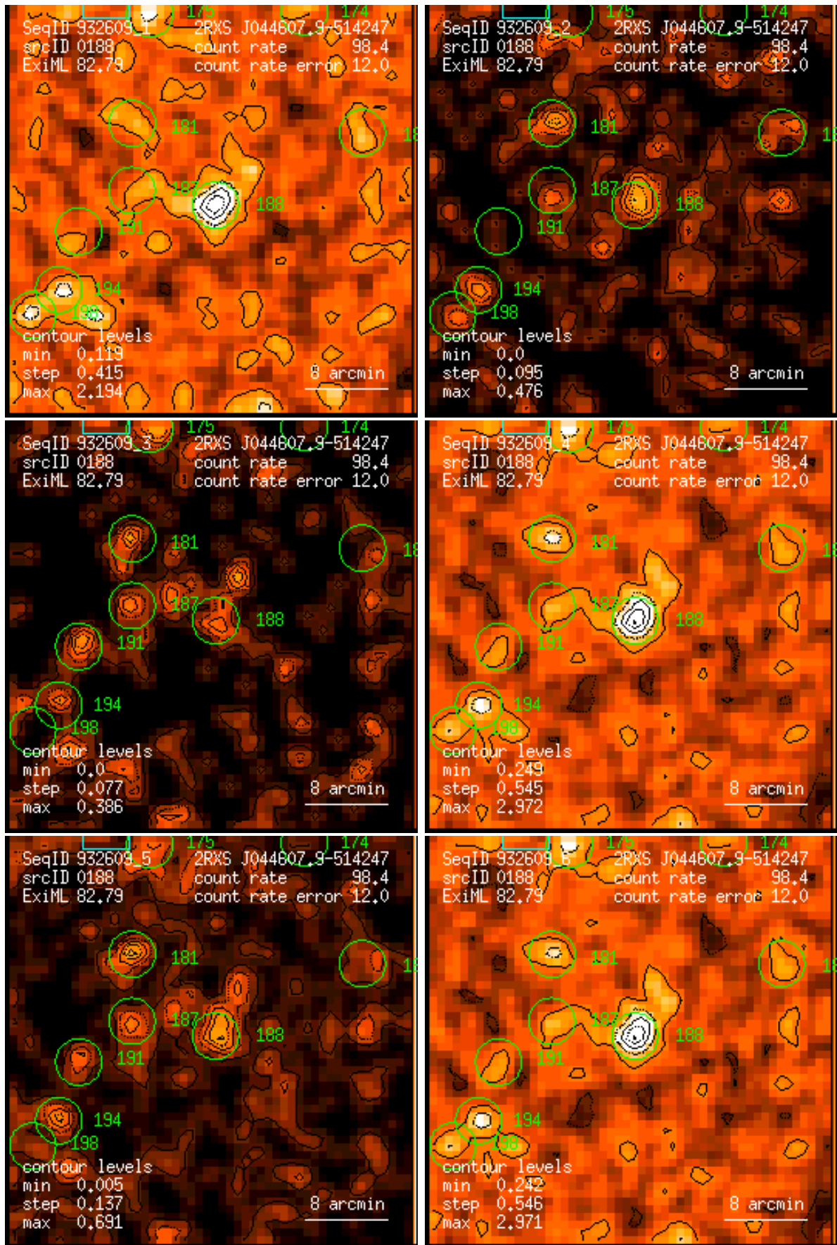
Figure 188: RASS 932609: detection 0188: band rate images, Gaussian filter: (1) PSPC channels 11 – 41, (2) 52 – 90, (3) 91 – 201, (4) 11 – 235, (5) 52 – 201, (6) 11 – 201. Broad band rates in counts/ks. Band rate contour levels in counts/ks/arcmin 2 .
