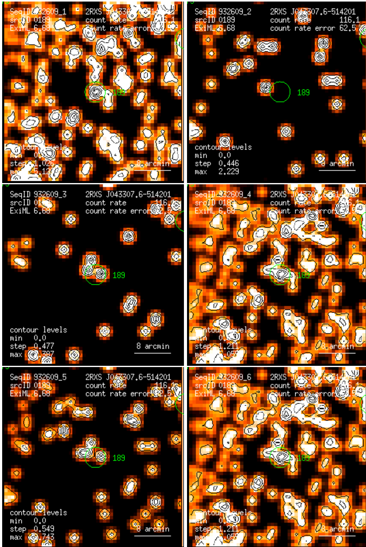
Figure 189: RASS 932609: detection 0189: band rate images, Gaussian filter: (1) PSPC channels 11 – 41, (2) 52 – 90, (3) 91 – 201, (4) 11 – 235, (5) 52 – 201, (6) 11 – 201. Broad band rates in counts/ks. Band rate contour levels in counts/ks/arcmin 2 .
