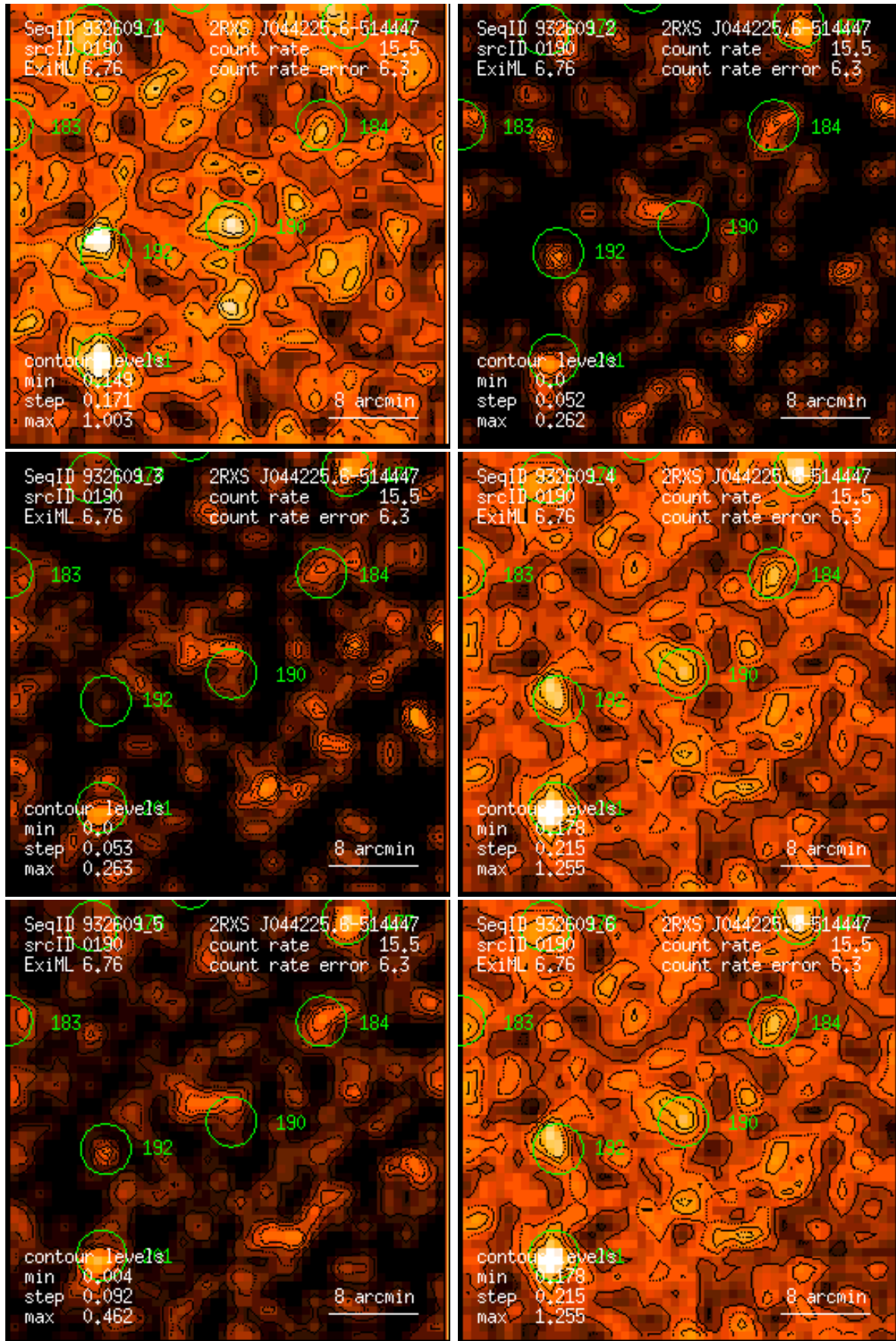
Figure 190: RASS 932609: detection 0190: band rate images, Gaussian filter: (1) PSPC channels 11 – 41, (2) 52 – 90, (3) 91 – 201, (4) 11 – 235, (5) 52 – 201, (6) 11 – 201. Broad band rates in counts/ks. Band rate contour levels in counts/ks/arcmin 2 .
