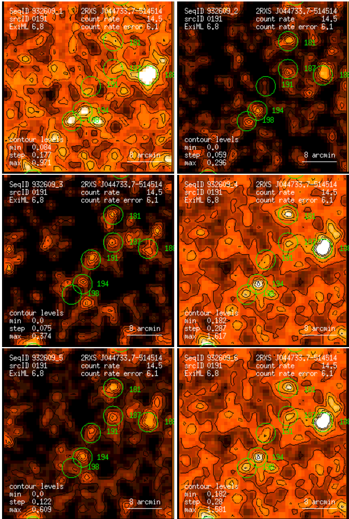
Figure 191: RASS 932609: detection 0191: band rate images, Gaussian filter: (1) PSPC channels 11 – 41, (2) 52 – 90, (3) 91 – 201, (4) 11 – 235, (5) 52 – 201, (6) 11 – 201. Broad band rates in counts/ks. Band rate contour levels in counts/ks/arcmin 2 .
