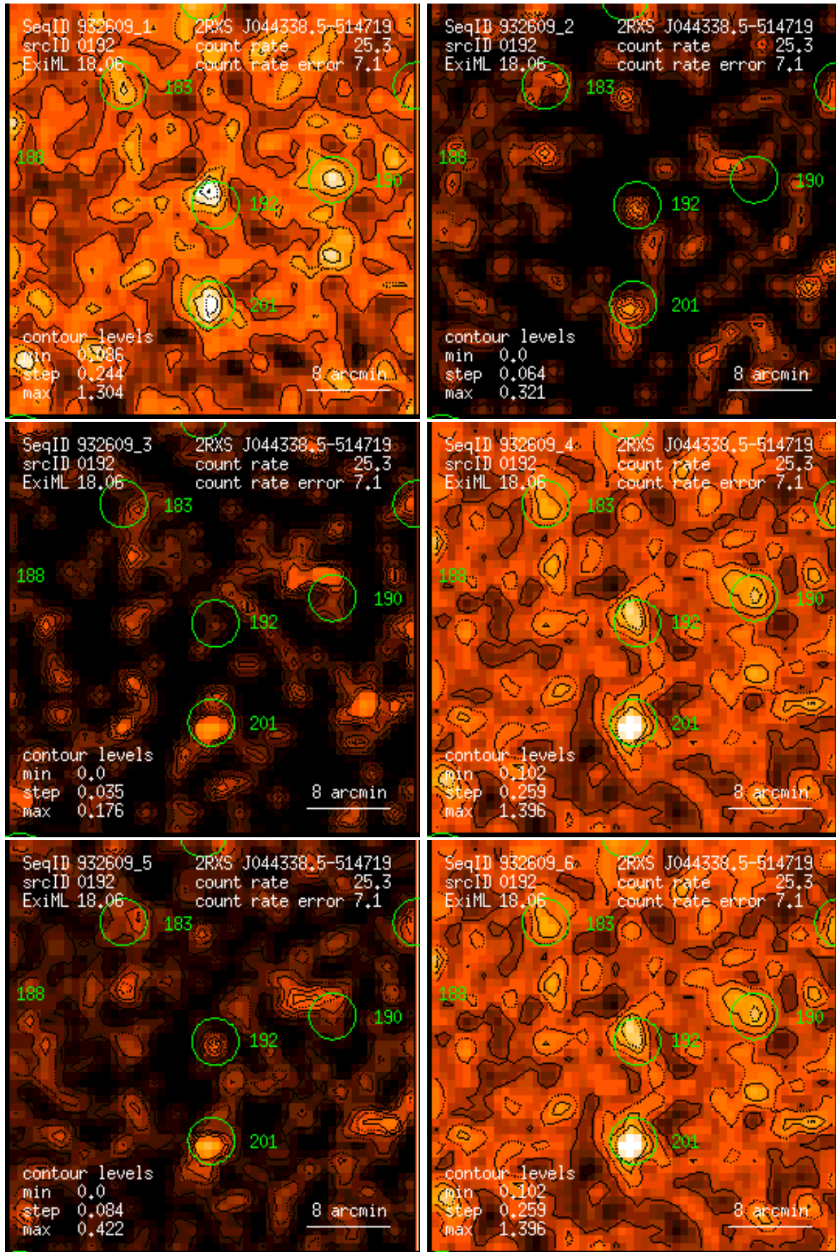
Figure 192: RASS 932609: detection 0192: band rate images, Gaussian filter: (1) PSPC channels 11 – 41, (2) 52 – 90, (3) 91 – 201, (4) 11 – 235, (5) 52 – 201, (6) 11 – 201. Broad band rates in counts/ks. Band rate contour levels in counts/ks/arcmin 2 .
