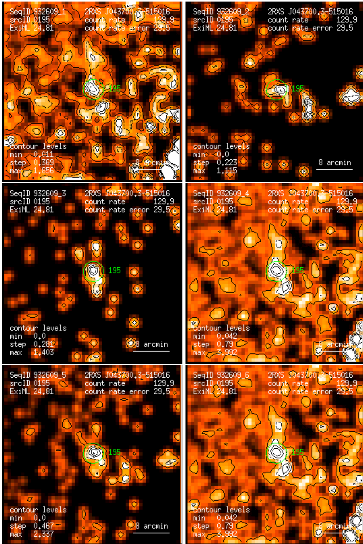
Figure 195: RASS 932609: detection 0195: band rate images, Gaussian filter: (1) PSPC channels 11 – 41, (2) 52 – 90, (3) 91 – 201, (4) 11 – 235, (5) 52 – 201, (6) 11 – 201. Broad band rates in counts/ks. Band rate contour levels in counts/ks/arcmin 2 .
